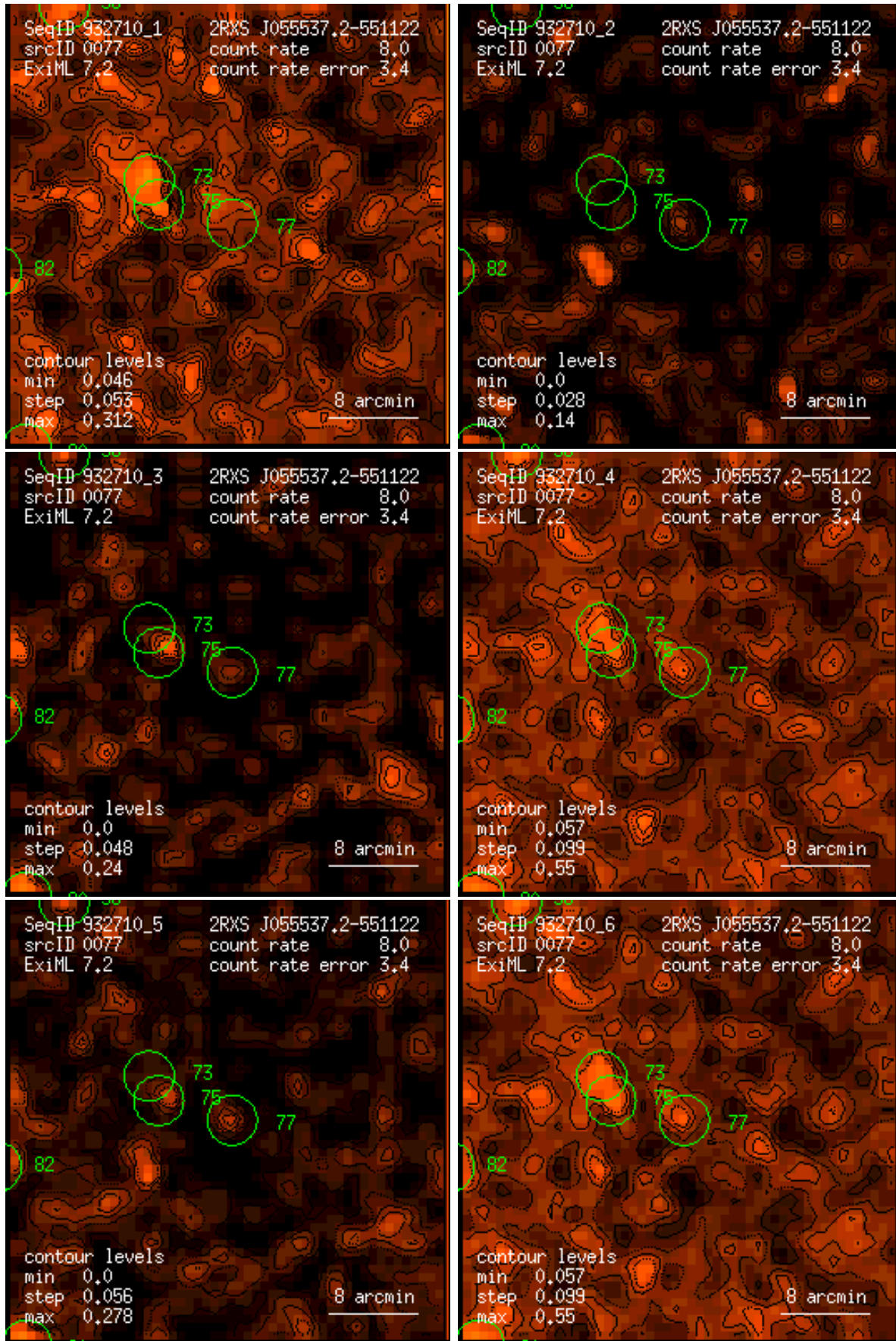
Figure 77: RASS 932710: detection 0077: band rate images, Gaussian filter: (1) PSPC channels 11 – 41, (2) 52 – 90, (3) 91 – 201, (4) 11 – 235, (5) 52 – 201, (6) 11 – 201. Broad band rates in counts/ks. Band rate contour levels in counts/ks/arcmin 2 .
