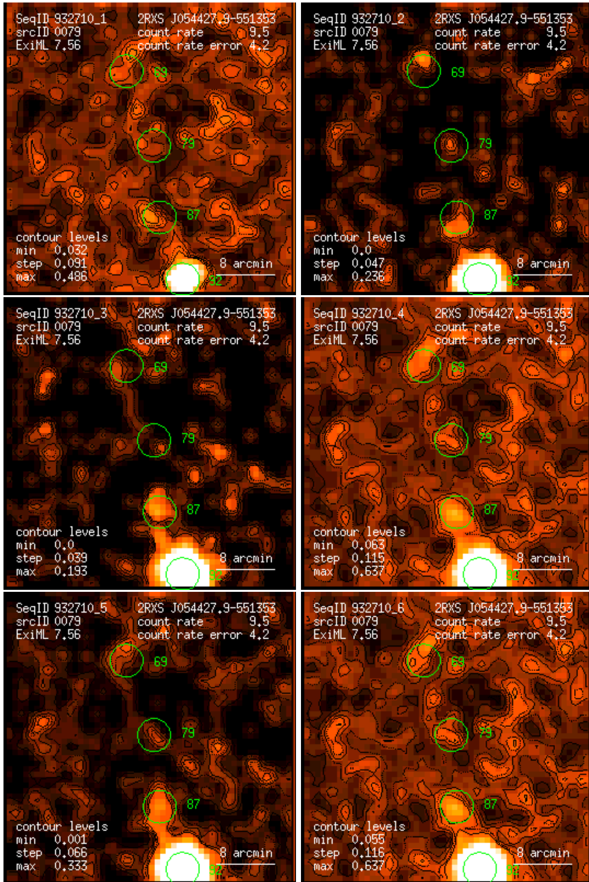
Figure 79: RASS 932710: detection 0079: band rate images, Gaussian filter: (1) PSPC channels 11 – 41, (2) 52 – 90, (3) 91 – 201, (4) 11 – 235, (5) 52 – 201, (6) 11 – 201. Broad band rates in counts/ks. Band rate contour levels in counts/ks/arcmin 2 .
