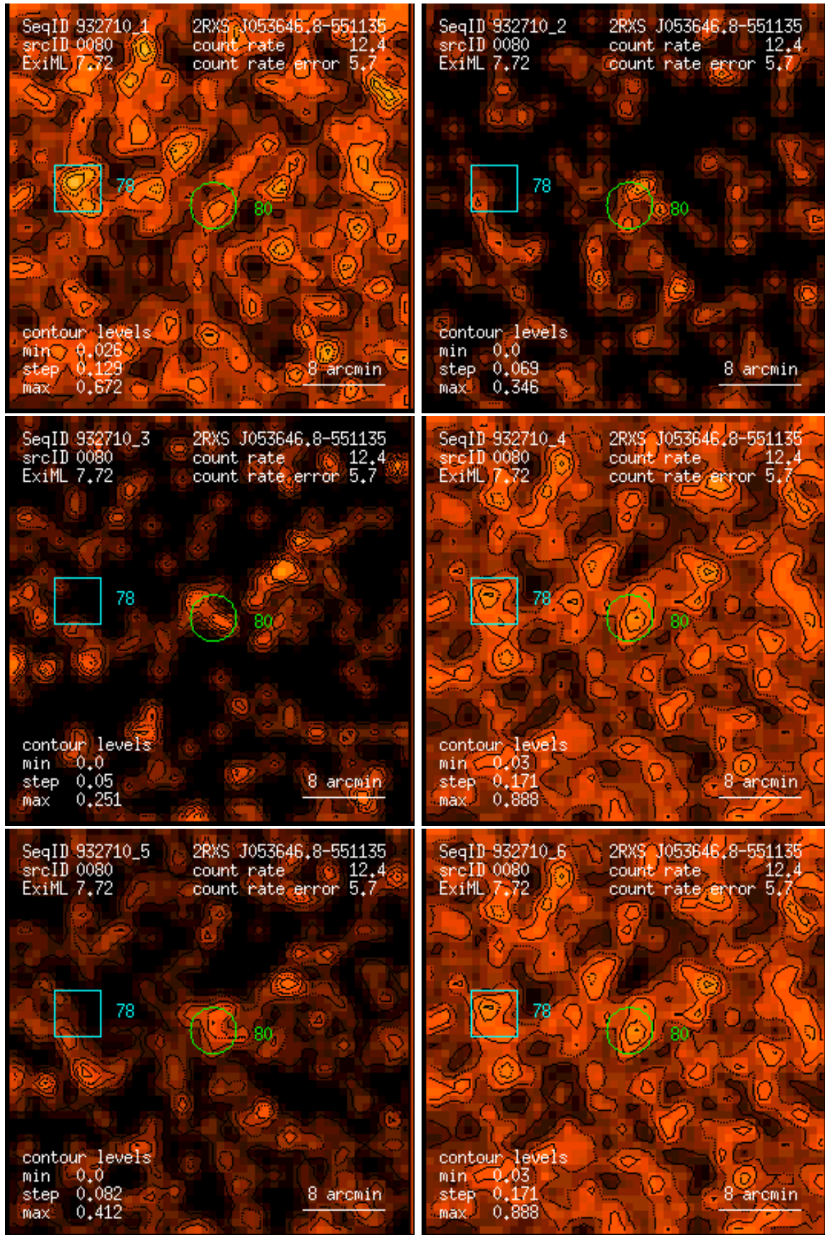
Figure 80: RASS 932710: detection 0080: band rate images, Gaussian filter: (1) PSPC channels 11 – 41, (2) 52 – 90, (3) 91 – 201, (4) 11 – 235, (5) 52 – 201, (6) 11 – 201. Broad band rates in counts/ks. Band rate contour levels in counts/ks/arcmin 2 .
