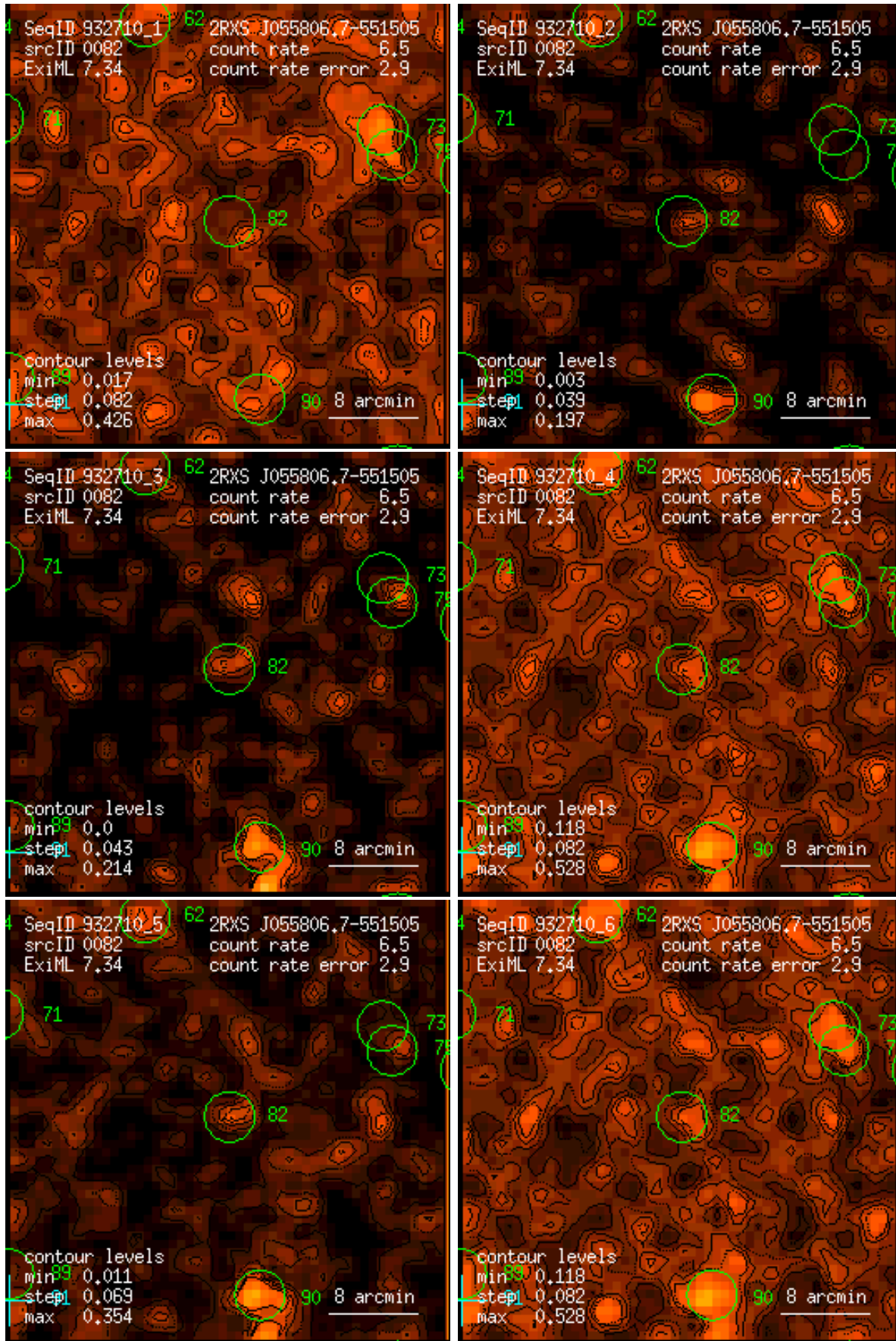
Figure 82: RASS 932710: detection 0082: band rate images, Gaussian filter: (1) PSPC channels 11 – 41, (2) 52 – 90, (3) 91 – 201, (4) 11 – 235, (5) 52 – 201, (6) 11 – 201. Broad band rates in counts/ks. Band rate contour levels in counts/ks/arcmin 2 .
