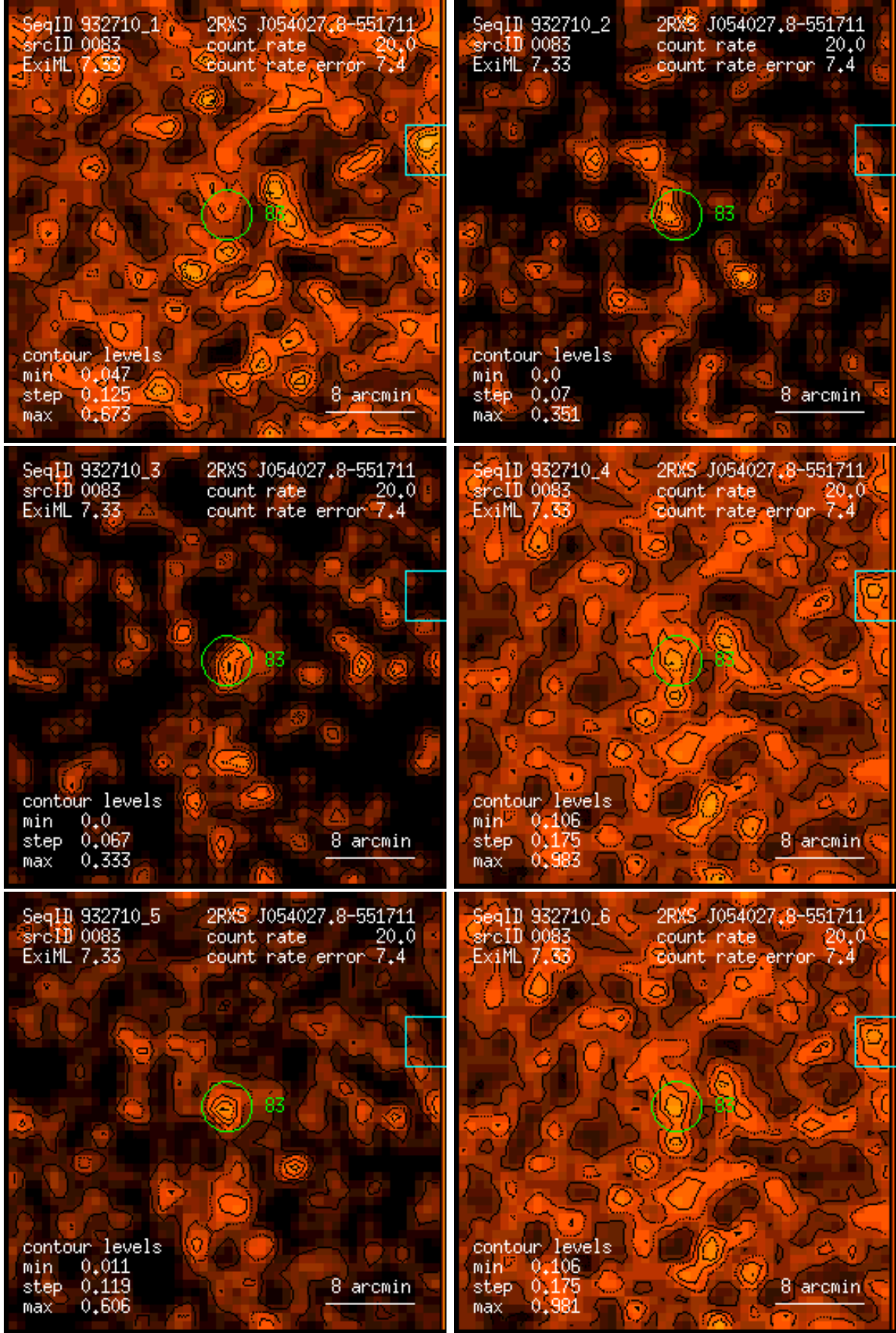
Figure 83: RASS 932710: detection 0083: band rate images, Gaussian filter: (1) PSPC channels 11 – 41, (2) 52 – 90, (3) 91 – 201, (4) 11 – 235, (5) 52 – 201, (6) 11 – 201. Broad band rates in counts/ks. Band rate contour levels in counts/ks/arcmin 2 .
