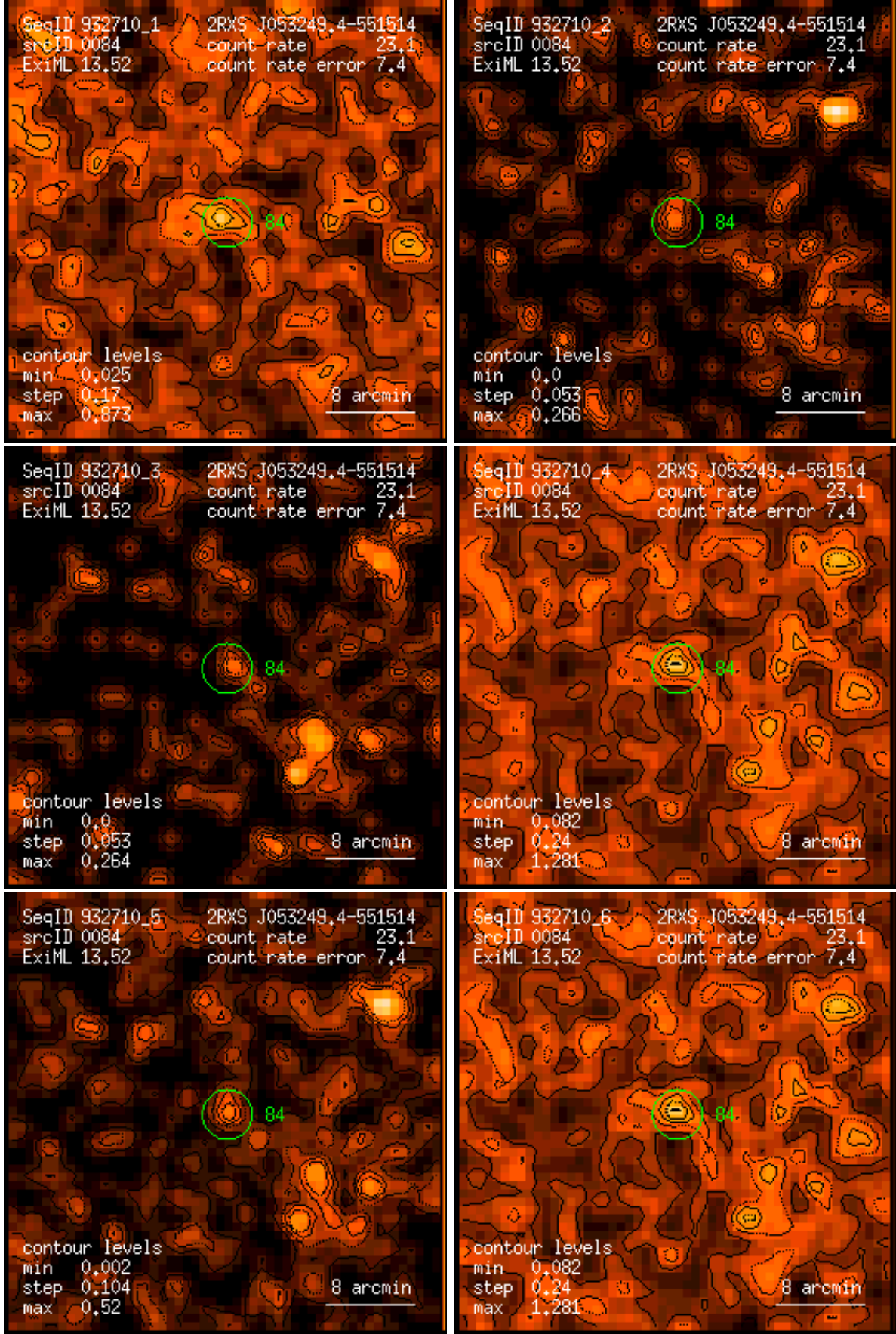
Figure 84: RASS 932710: detection 0084: band rate images, Gaussian filter: (1) PSPC channels 11 – 41, (2) 52 – 90, (3) 91 – 201, (4) 11 – 235, (5) 52 – 201, (6) 11 – 201. Broad band rates in counts/ks. Band rate contour levels in counts/ks/arcmin 2 .
