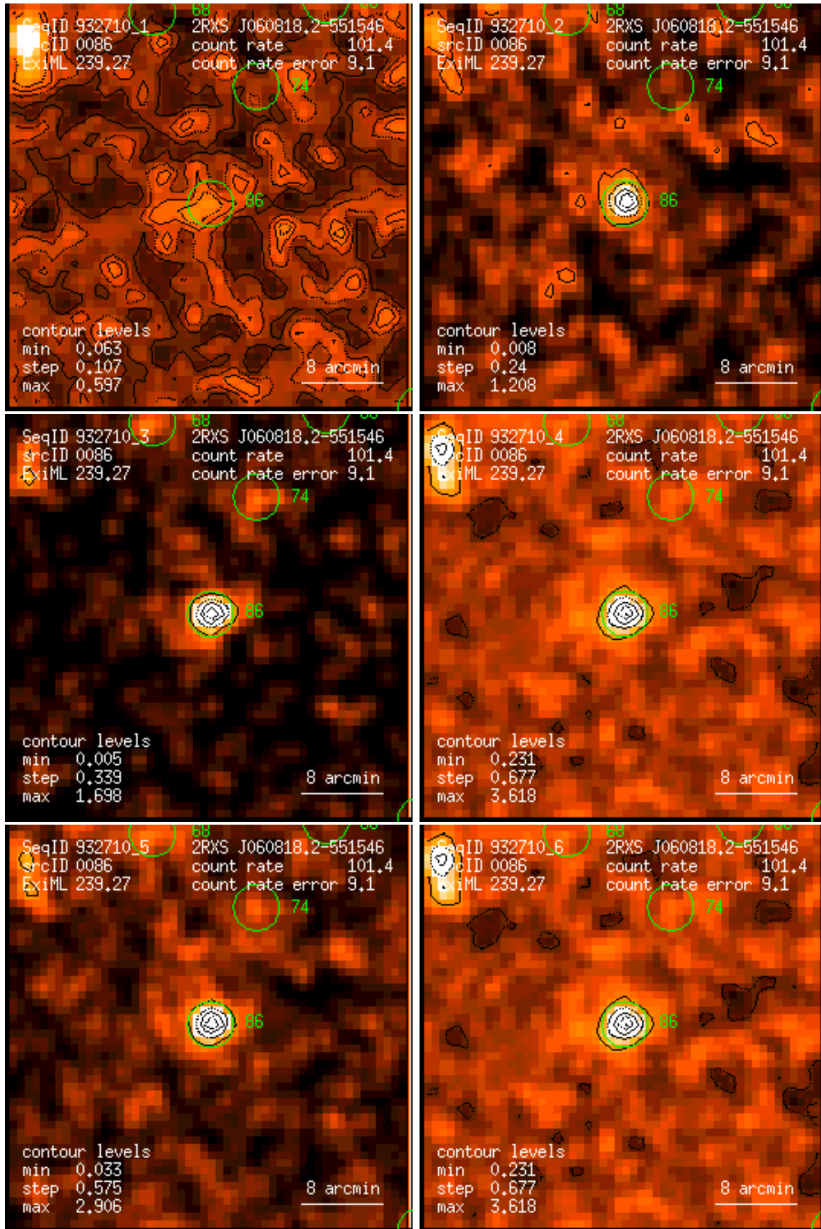
Figure 86: RASS 932710: detection 0086: band rate images, Gaussian filter: (1) PSPC channels 11 – 41, (2) 52 – 90, (3) 91 – 201, (4) 11 – 235, (5) 52 – 201, (6) 11 – 201. Broad band rates in counts/ks. Band rate contour levels in counts/ks/arcmin 2 .
