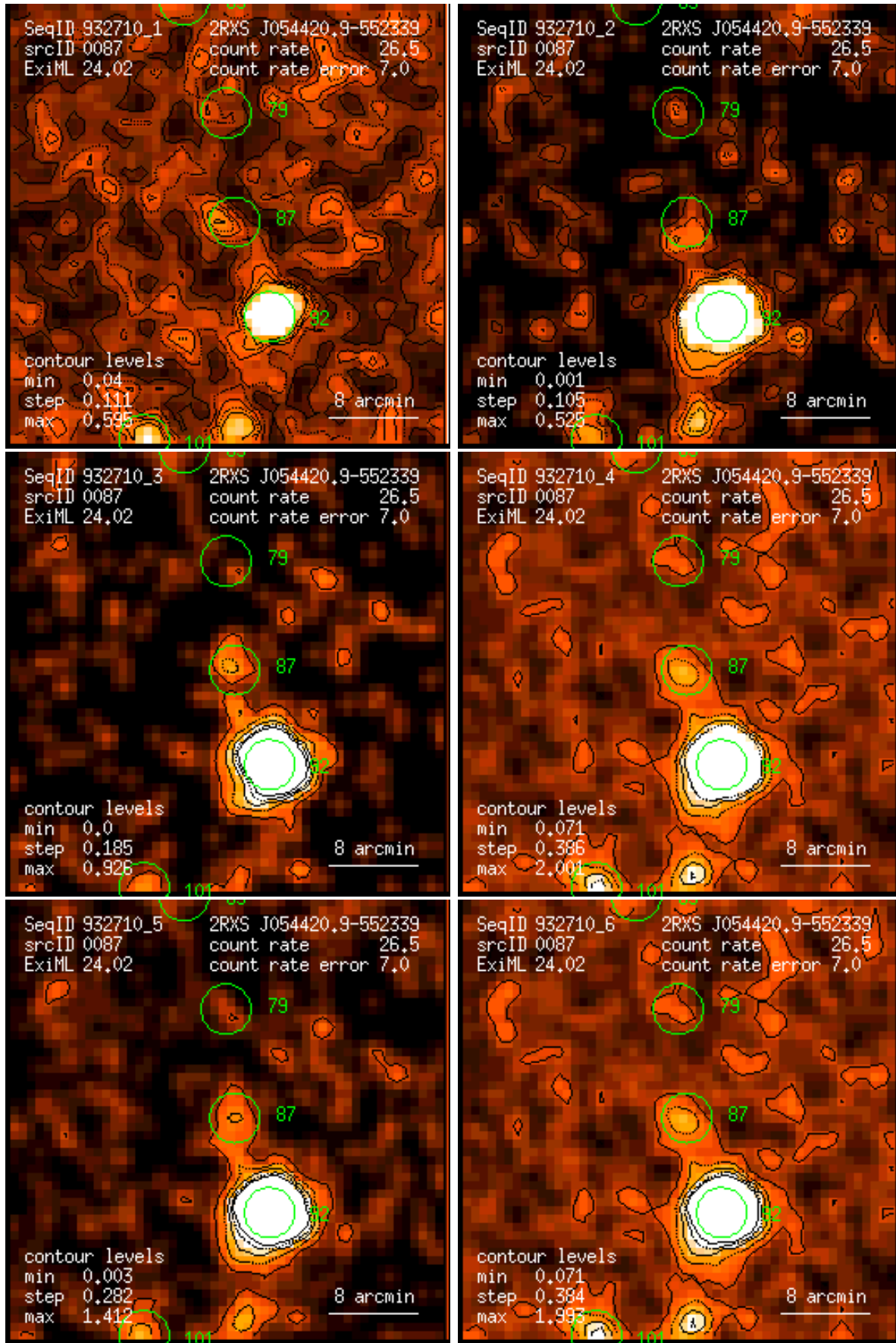
Figure 87: RASS 932710: detection 0087: band rate images, Gaussian filter: (1) PSPC channels 11 – 41, (2) 52 – 90, (3) 91 – 201, (4) 11 – 235, (5) 52 – 201, (6) 11 – 201. Broad band rates in counts/ks. Band rate contour levels in counts/ks/arcmin 2 .
