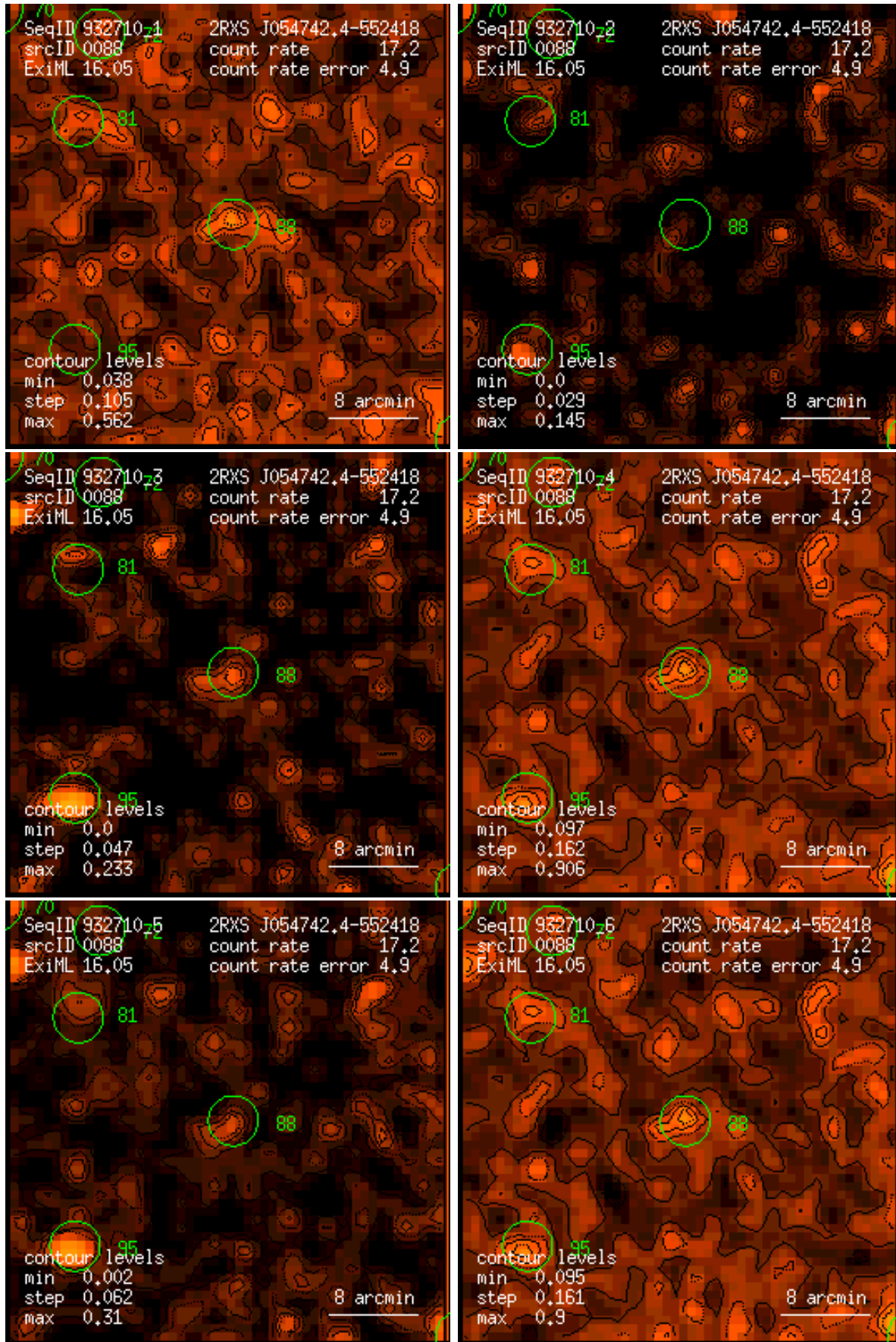
Figure 88: RASS 932710: detection 0088: band rate images, Gaussian filter: (1) PSPC channels 11 – 41, (2) 52 – 90, (3) 91 – 201, (4) 11 – 235, (5) 52 – 201, (6) 11 – 201. Broad band rates in counts/ks. Band rate contour levels in counts/ks/arcmin 2 .
