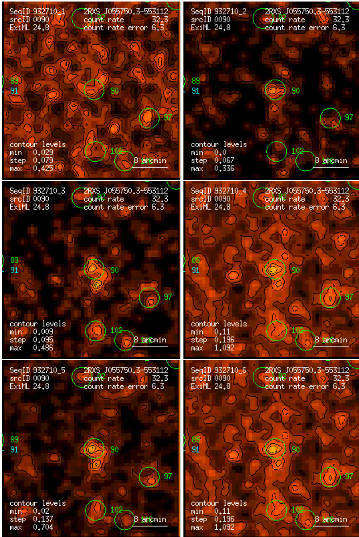
Figure 90: RASS 932710: detection 0090: band rate images, Gaussian filter: (1) PSPC channels 11 – 41, (2) 52 – 90, (3) 91 – 201, (4) 11 – 235, (5) 52 – 201, (6) 11 – 201. Broad band rates in counts/ks. Band rate contour levels in counts/ks/arcmin 2 .
