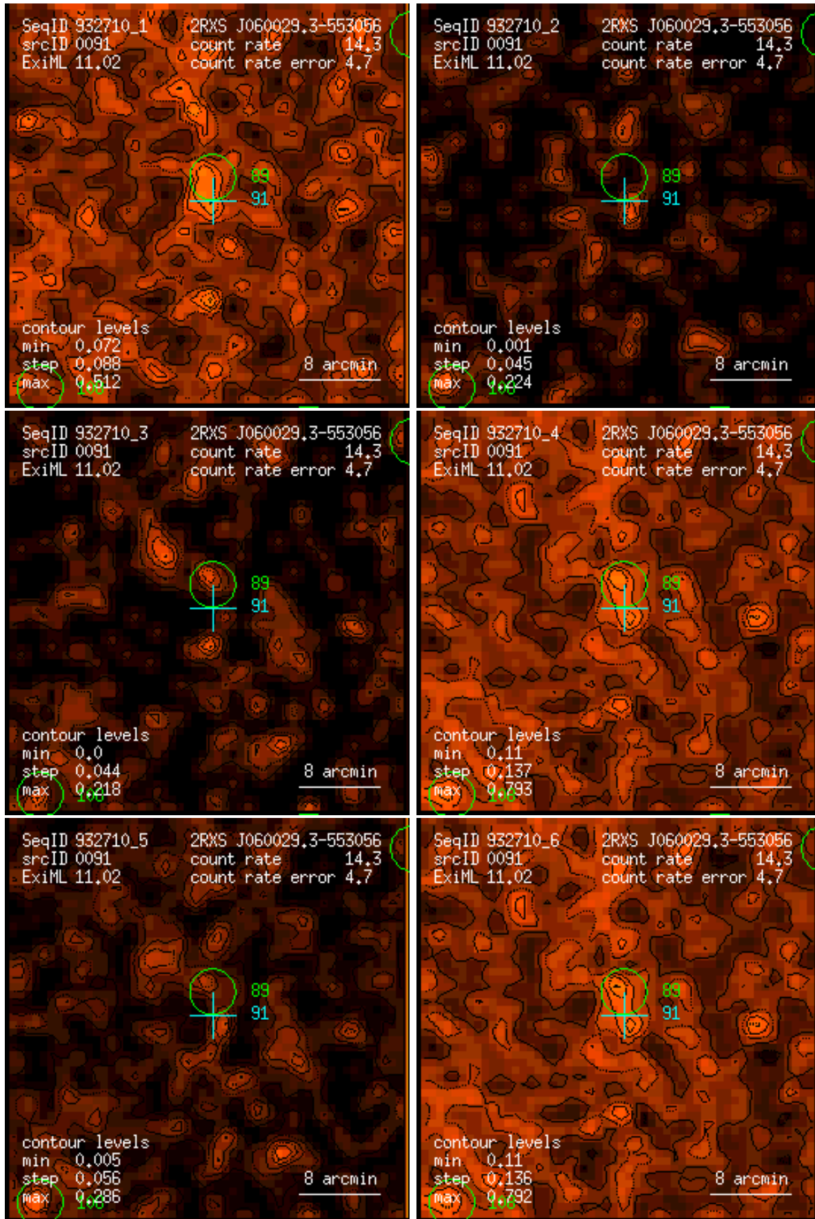
Figure 91: RASS 932710: detection 0091: band rate images, Gaussian filter: (1) PSPC channels 11 – 41, (2) 52 – 90, (3) 91 – 201, (4) 11 – 235, (5) 52 – 201, (6) 11 – 201. Broad band rates in counts/ks. Band rate contour levels in counts/ks/arcmin 2 .
