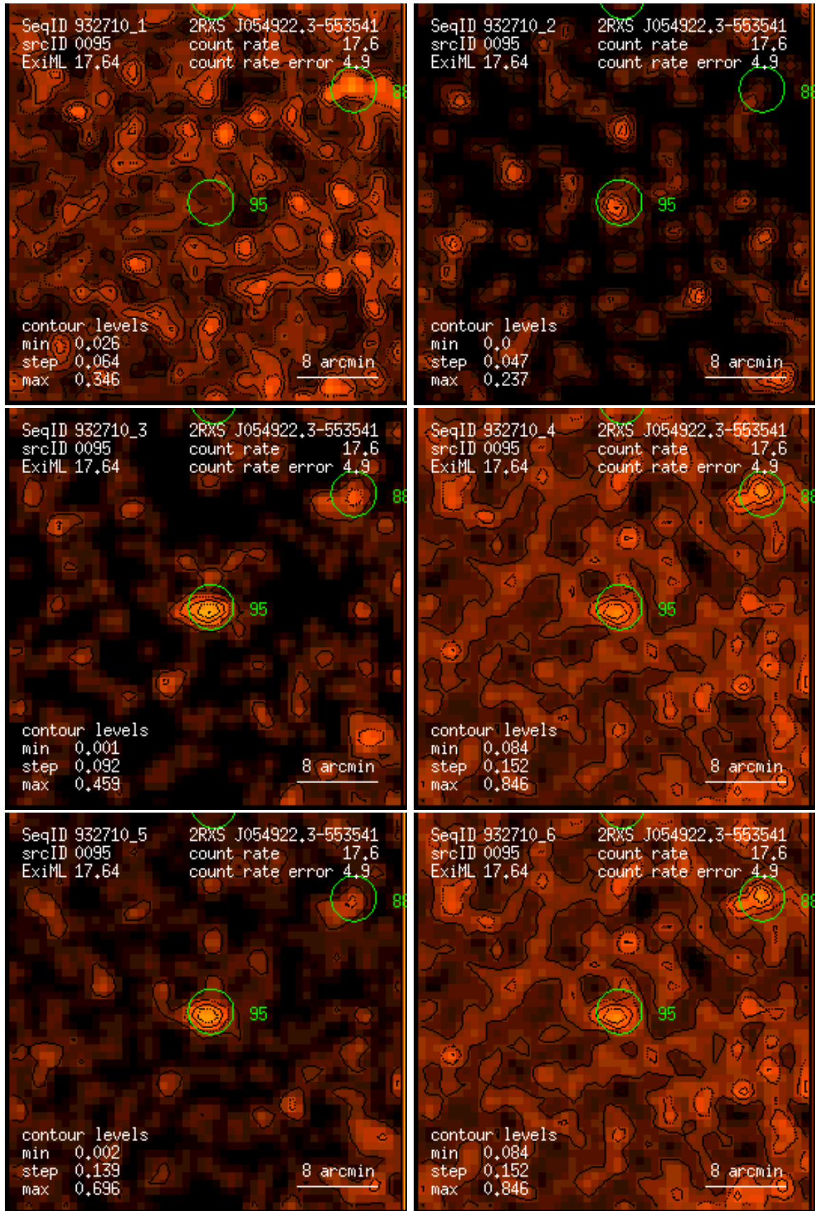
Figure 95: RASS 932710: detection 0095: band rate images, Gaussian filter: (1) PSPC channels 11 – 41, (2) 52 – 90, (3) 91 – 201, (4) 11 – 235, (5) 52 – 201, (6) 11 – 201. Broad band rates in counts/ks. Band rate contour levels in counts/ks/arcmin 2 .
