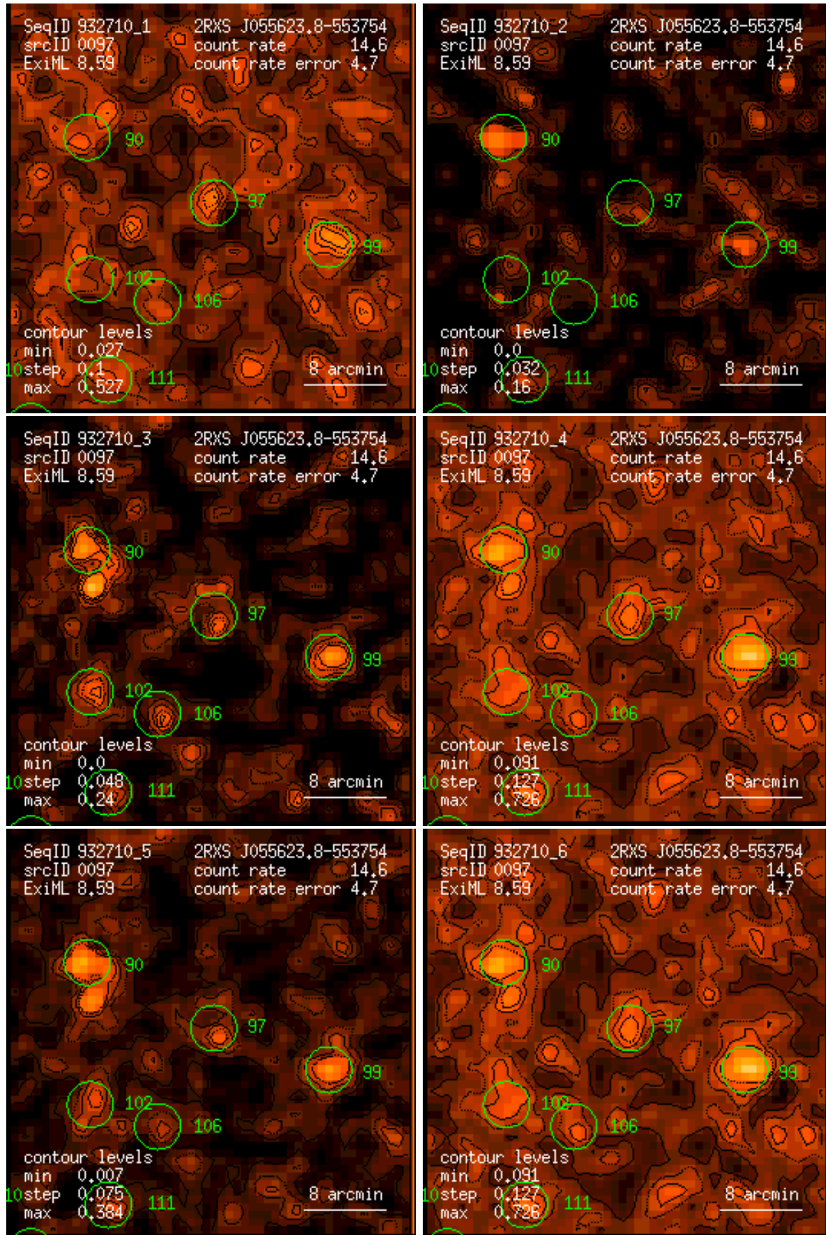
Figure 97: RASS 932710: detection 0097: band rate images, Gaussian filter: (1) PSPC channels 11 – 41, (2) 52 – 90, (3) 91 – 201, (4) 11 – 235, (5) 52 – 201, (6) 11 – 201. Broad band rates in counts/ks. Band rate contour levels in counts/ks/arcmin 2 .
