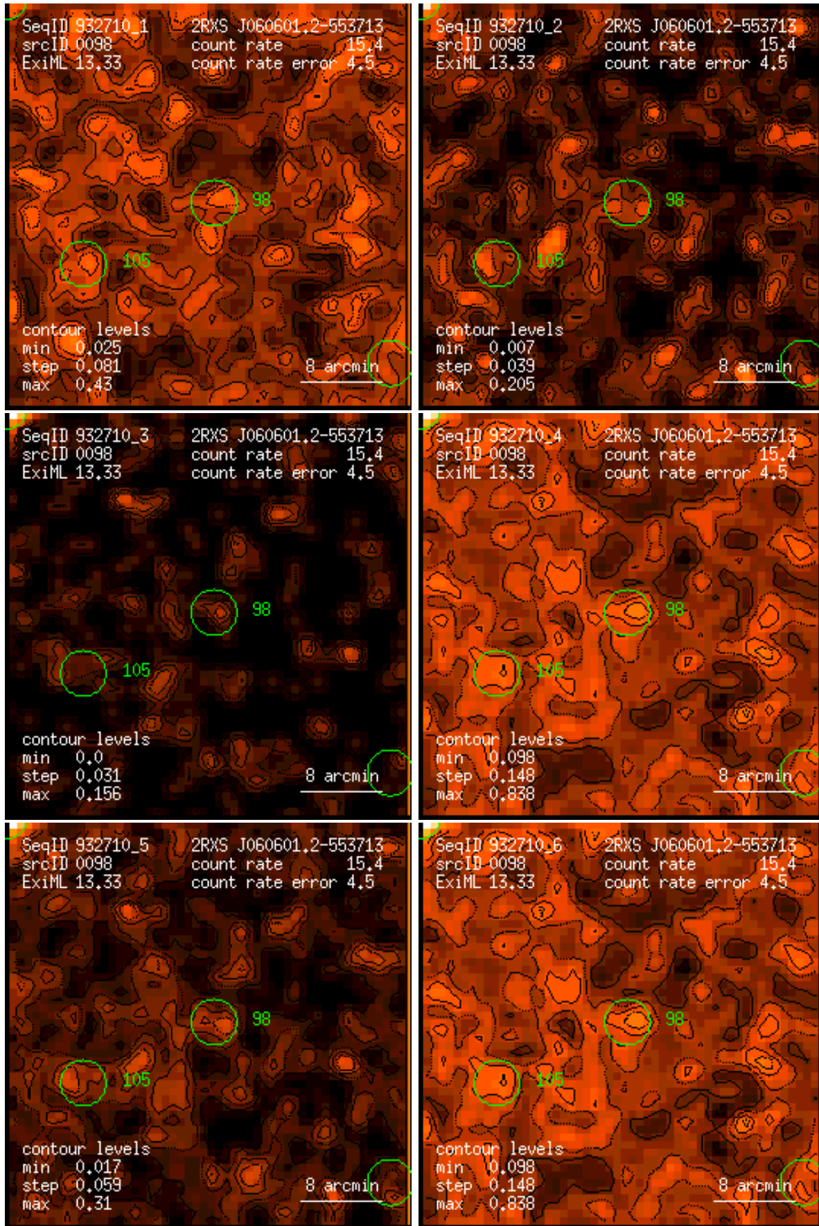
Figure 98: RASS 932710: detection 0098: band rate images, Gaussian filter: (1) PSPC channels 11 – 41, (2) 52 – 90, (3) 91 – 201, (4) 11 – 235, (5) 52 – 201, (6) 11 – 201. Broad band rates in counts/ks. Band rate contour levels in counts/ks/arcmin 2 .
