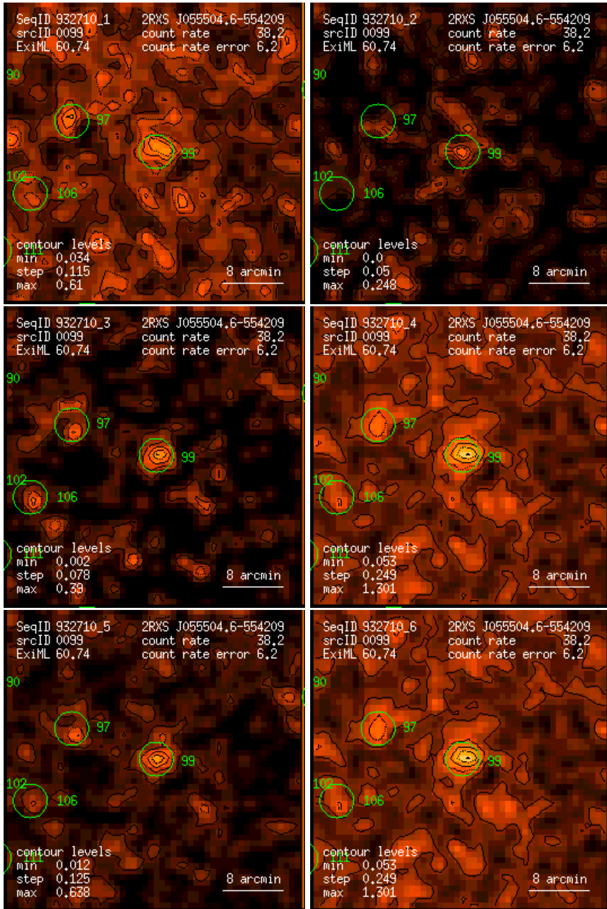
Figure 99: RASS 932710: detection 0099: band rate images, Gaussian filter: (1) PSPC channels 11 – 41, (2) 52 – 90, (3) 91 – 201, (4) 11 – 235, (5) 52 – 201, (6) 11 – 201. Broad band rates in counts/ks. Band rate contour levels in counts/ks/arcmin 2 .
