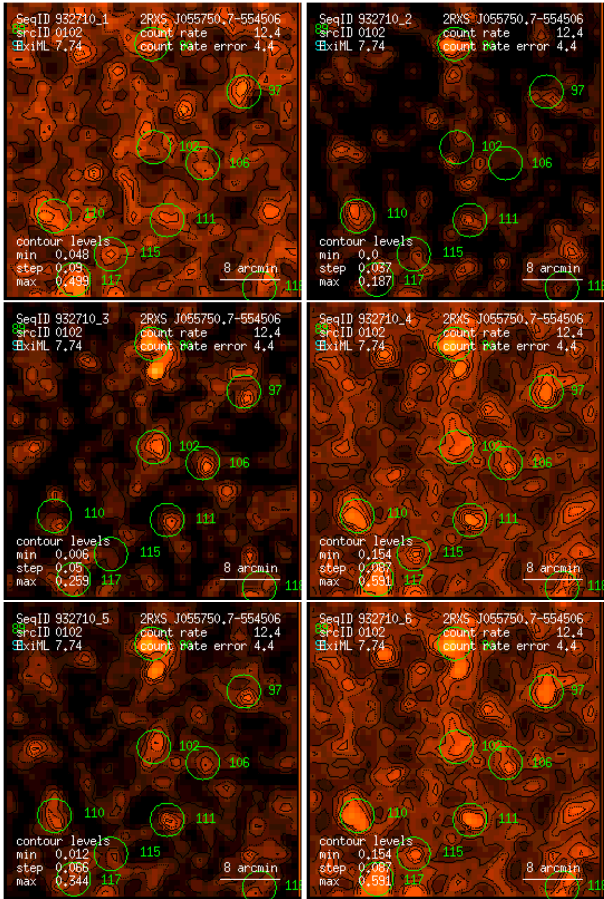
Figure 102: RASS 932710: detection 0102: band rate images, Gaussian filter: (1) PSPC channels 11 – 41, (2) 52 – 90, (3) 91 – 201, (4) 11 – 235, (5) 52 – 201, (6) 11 – 201. Broad band rates in counts/ks. Band rate contour levels in counts/ks/arcmin 2 .
