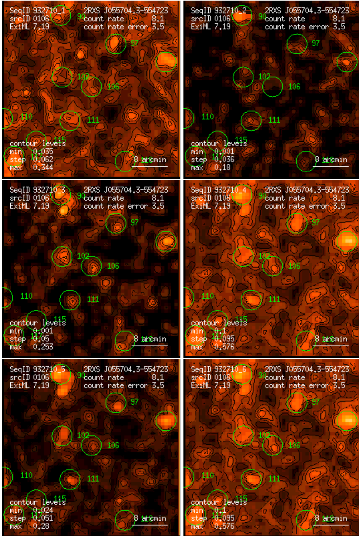
Figure 106: RASS 932710: detection 0106: band rate images, Gaussian filter: (1) PSPC channels 11 – 41, (2) 52 – 90, (3) 91 – 201, (4) 11 – 235, (5) 52 – 201, (6) 11 – 201. Broad band rates in counts/ks. Band rate contour levels in counts/ks/arcmin 2 .
