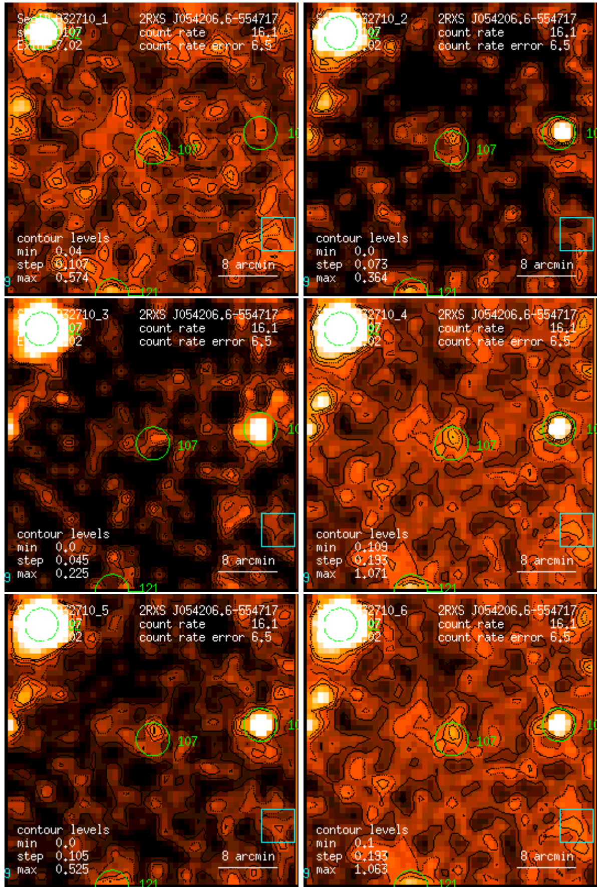
Figure 107: RASS 932710: detection 0107: band rate images, Gaussian filter: (1) PSPC channels 11 – 41, (2) 52 – 90, (3) 91 – 201, (4) 11 – 235, (5) 52 – 201, (6) 11 – 201. Broad band rates in counts/ks. Band rate contour levels in counts/ks/arcmin 2 .
