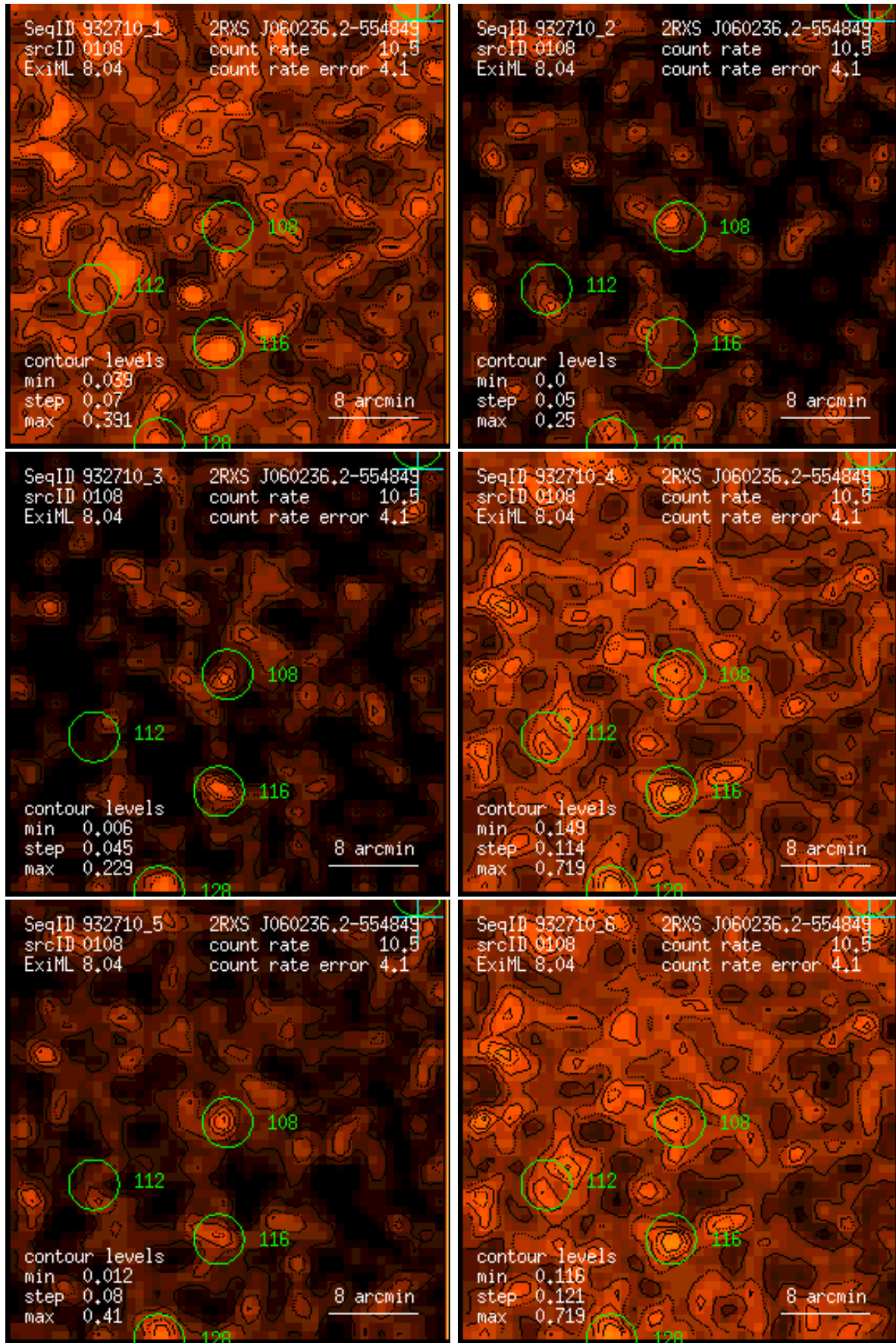
Figure 108: RASS 932710: detection 0108: band rate images, Gaussian filter: (1) PSPC channels 11 – 41, (2) 52 – 90, (3) 91 – 201, (4) 11 – 235, (5) 52 – 201, (6) 11 – 201. Broad band rates in counts/ks. Band rate contour levels in counts/ks/arcmin 2 .
