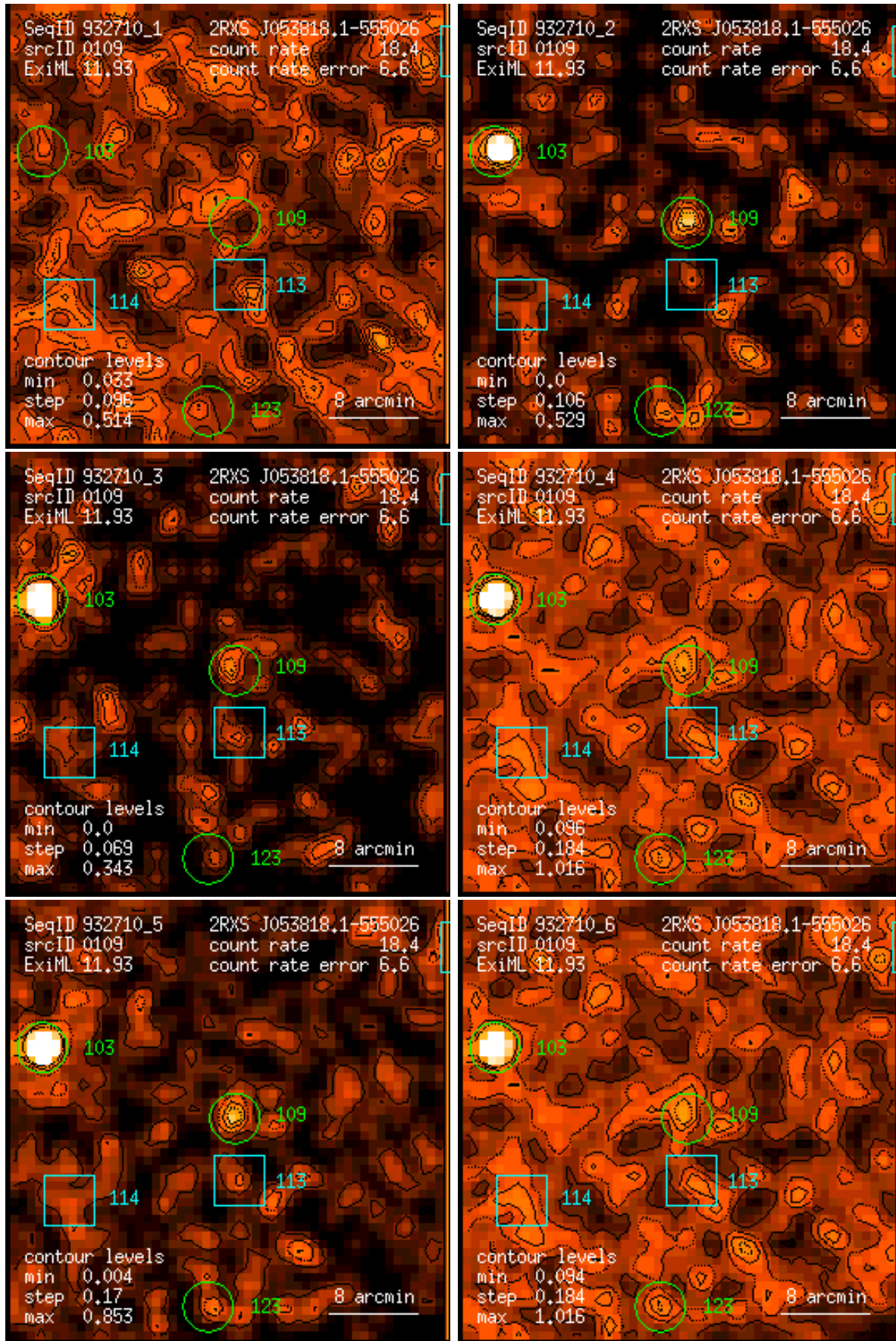
Figure 109: RASS 932710: detection 0109: band rate images, Gaussian filter: (1) PSPC channels 11 – 41, (2) 52 – 90, (3) 91 – 201, (4) 11 – 235, (5) 52 – 201, (6) 11 – 201. Broad band rates in counts/ks. Band rate contour levels in counts/ks/arcmin 2 .
