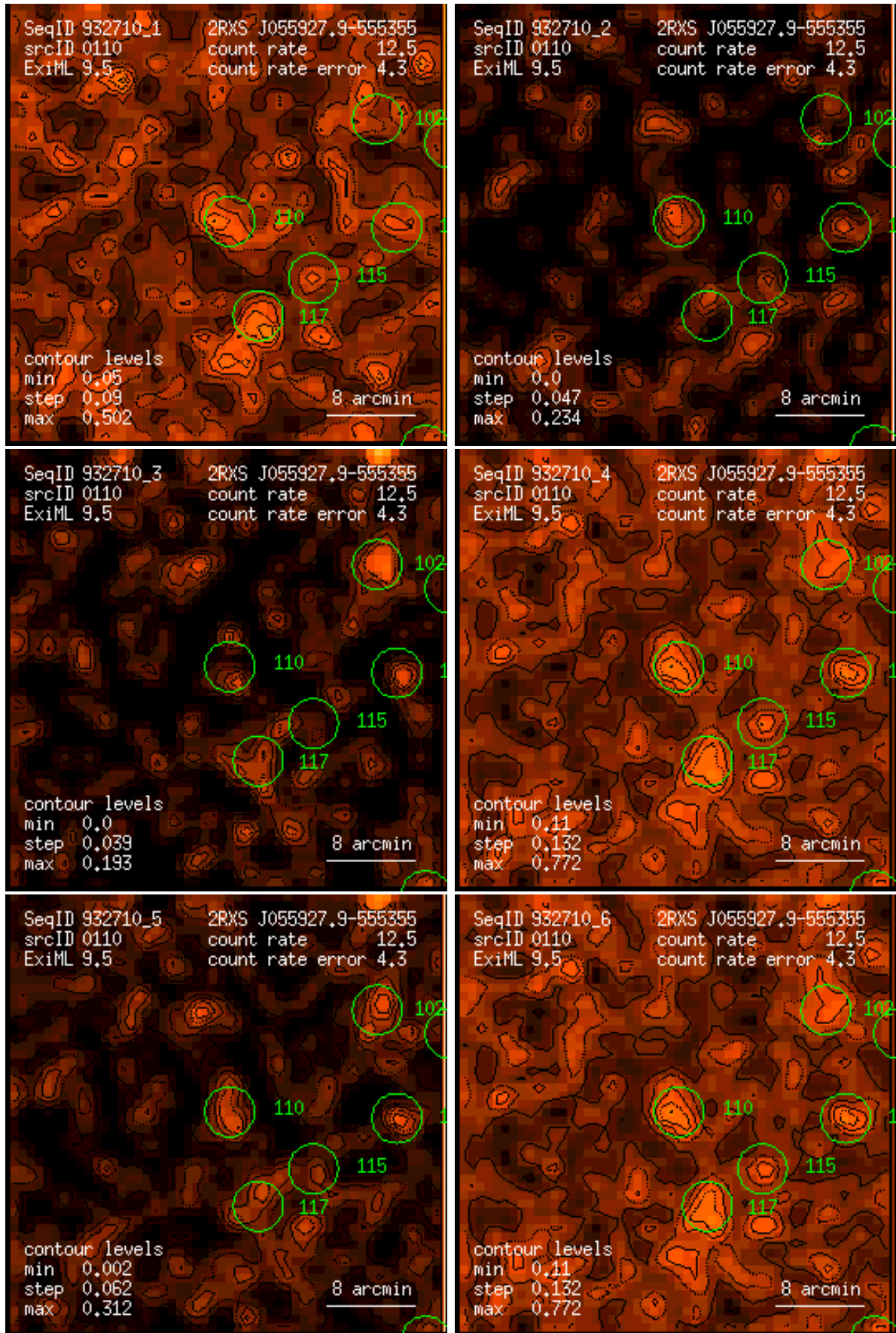
Figure 110: RASS 932710: detection 0110: band rate images, Gaussian filter: (1) PSPC channels 11 – 41, (2) 52 – 90, (3) 91 – 201, (4) 11 – 235, (5) 52 – 201, (6) 11 – 201. Broad band rates in counts/ks. Band rate contour levels in counts/ks/arcmin 2 .
