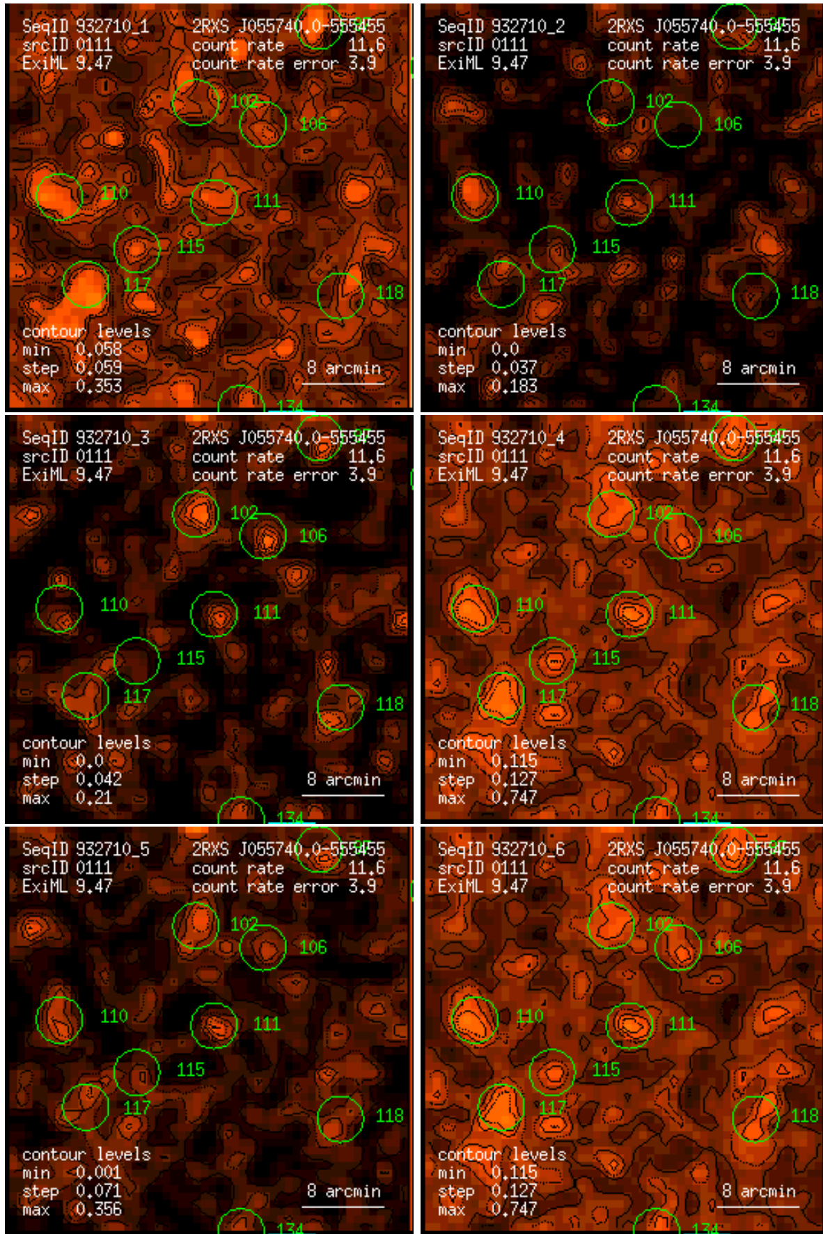
Figure 111: RASS 932710: detection 0111: band rate images, Gaussian filter: (1) PSPC channels 11 – 41, (2) 52 – 90, (3) 91 – 201, (4) 11 – 235, (5) 52 – 201, (6) 11 – 201. Broad band rates in counts/ks. Band rate contour levels in counts/ks/arcmin 2 .
