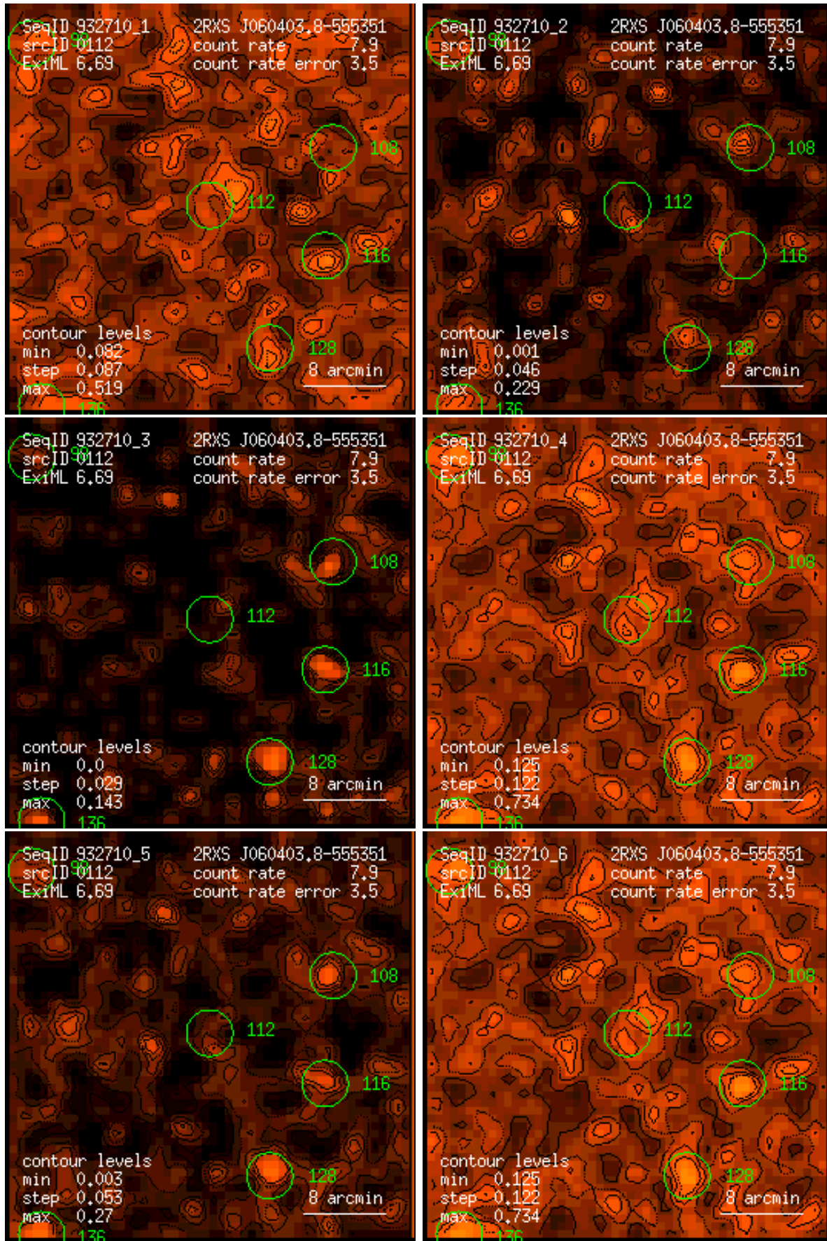
Figure 112: RASS 932710: detection 0112: band rate images, Gaussian filter: (1) PSPC channels 11 – 41, (2) 52 – 90, (3) 91 – 201, (4) 11 – 235, (5) 52 – 201, (6) 11 – 201. Broad band rates in counts/ks. Band rate contour levels in counts/ks/arcmin 2 .
