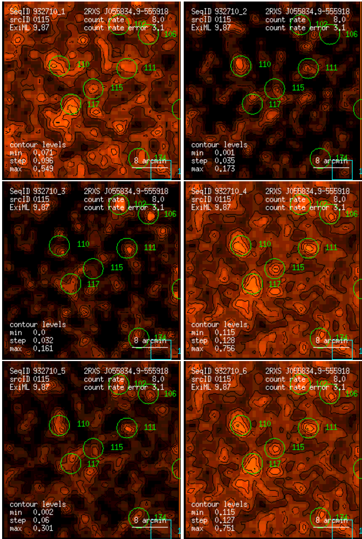
Figure 115: RASS 932710: detection 0115: band rate images, Gaussian filter: (1) PSPC channels 11 – 41, (2) 52 – 90, (3) 91 – 201, (4) 11 – 235, (5) 52 – 201, (6) 11 – 201. Broad band rates in counts/ks. Band rate contour levels in counts/ks/arcmin 2 .
