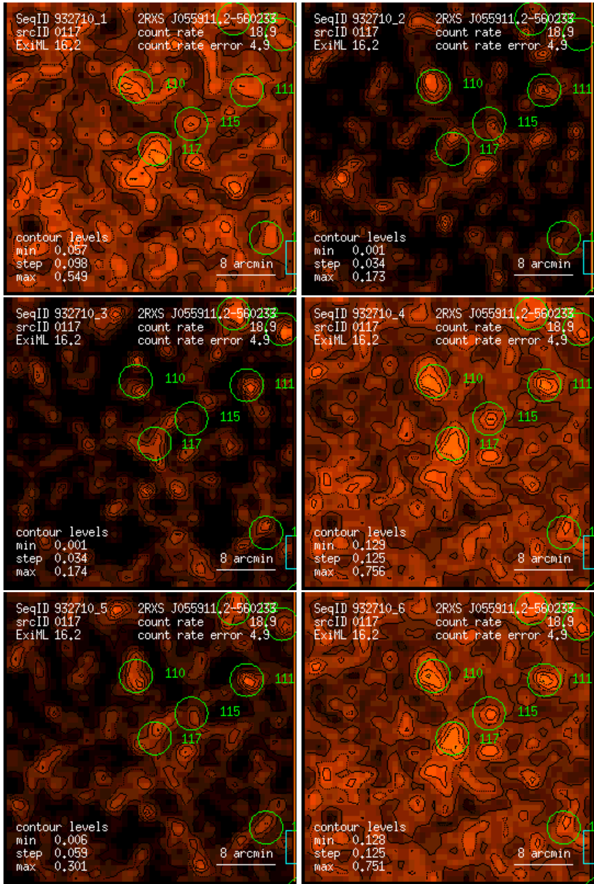
Figure 117: RASS 932710: detection 0117: band rate images, Gaussian filter: (1) PSPC channels 11 – 41, (2) 52 – 90, (3) 91 – 201, (4) 11 – 235, (5) 52 – 201, (6) 11 – 201. Broad band rates in counts/ks. Band rate contour levels in counts/ks/arcmin 2 .
