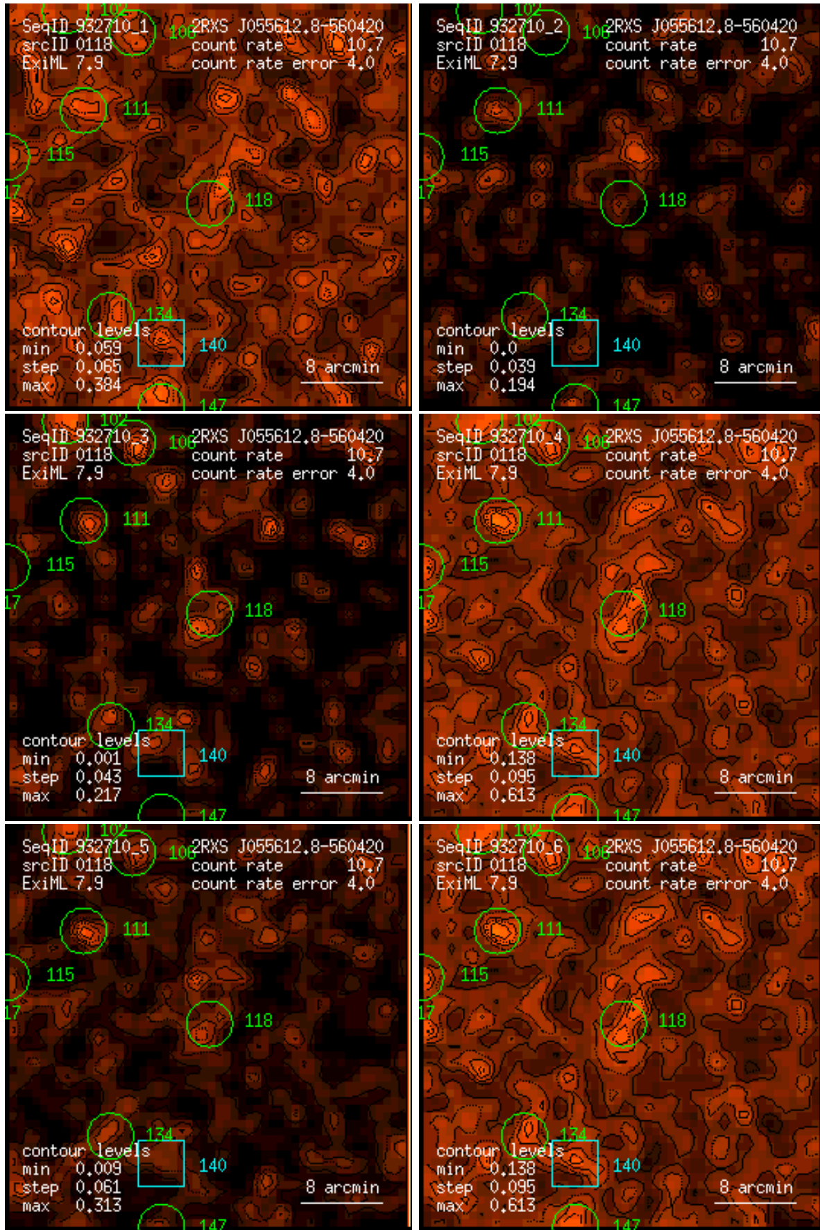
Figure 118: RASS 932710: detection 0118: band rate images, Gaussian filter: (1) PSPC channels 11 – 41, (2) 52 – 90, (3) 91 – 201, (4) 11 – 235, (5) 52 – 201, (6) 11 – 201. Broad band rates in counts/ks. Band rate contour levels in counts/ks/arcmin 2 .
