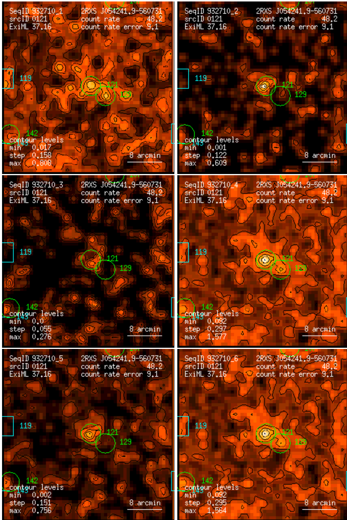
Figure 121: RASS 932710: detection 0121: band rate images, Gaussian filter: (1) PSPC channels 11 – 41, (2) 52 – 90, (3) 91 – 201, (4) 11 – 235, (5) 52 – 201, (6) 11 – 201. Broad band rates in counts/ks. Band rate contour levels in counts/ks/arcmin 2 .
