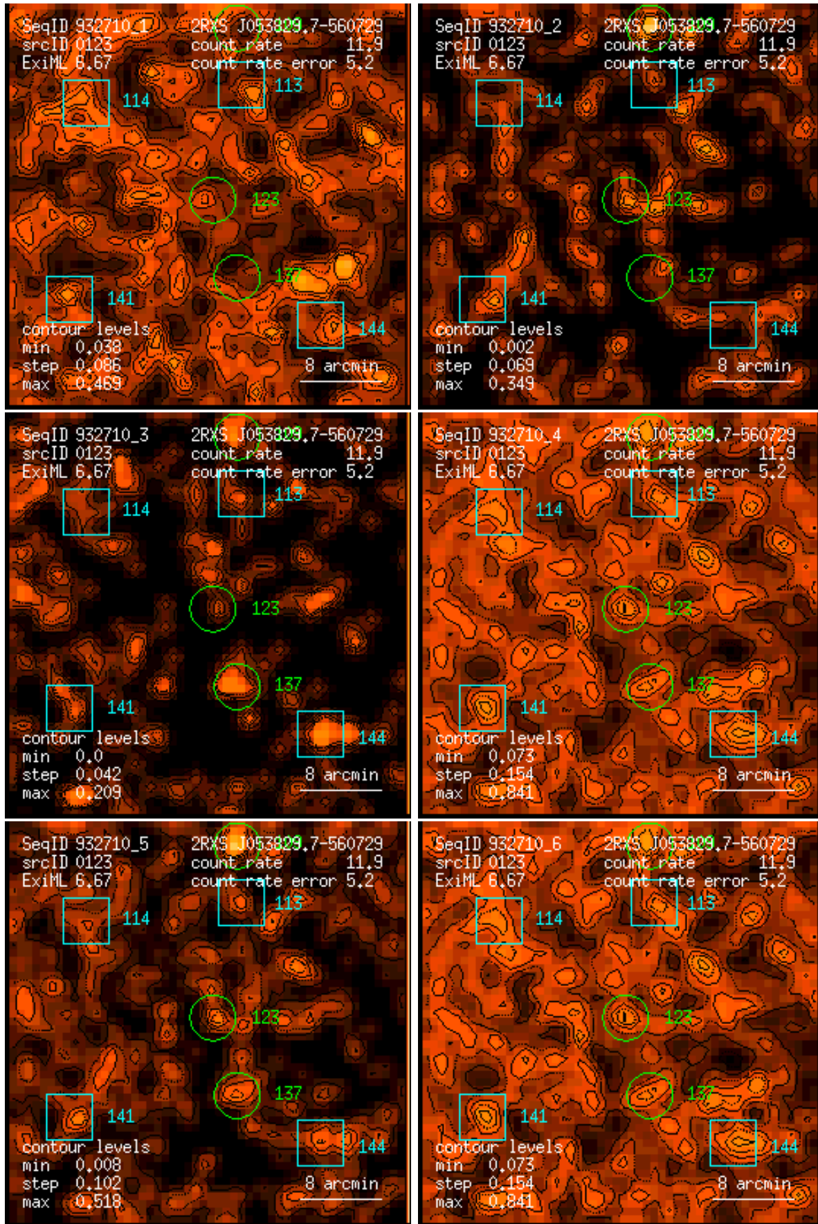
Figure 123: RASS 932710: detection 0123: band rate images, Gaussian filter: (1) PSPC channels 11 – 41, (2) 52 – 90, (3) 91 – 201, (4) 11 – 235, (5) 52 – 201, (6) 11 – 201. Broad band rates in counts/ks. Band rate contour levels in counts/ks/arcmin 2 .
