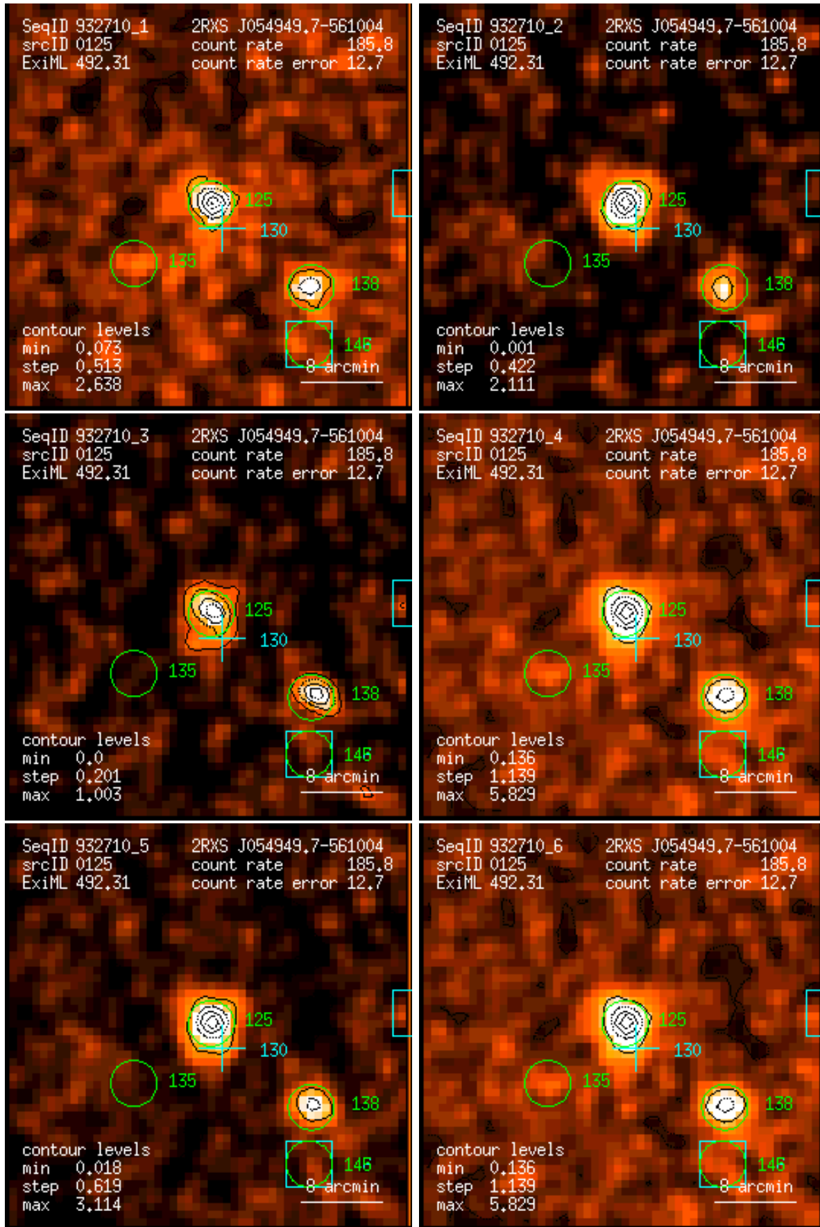
Figure 125: RASS 932710: detection 0125: band rate images, Gaussian filter: (1) PSPC channels 11 – 41, (2) 52 – 90, (3) 91 – 201, (4) 11 – 235, (5) 52 – 201, (6) 11 – 201. Broad band rates in counts/ks. Band rate contour levels in counts/ks/arcmin 2 .
