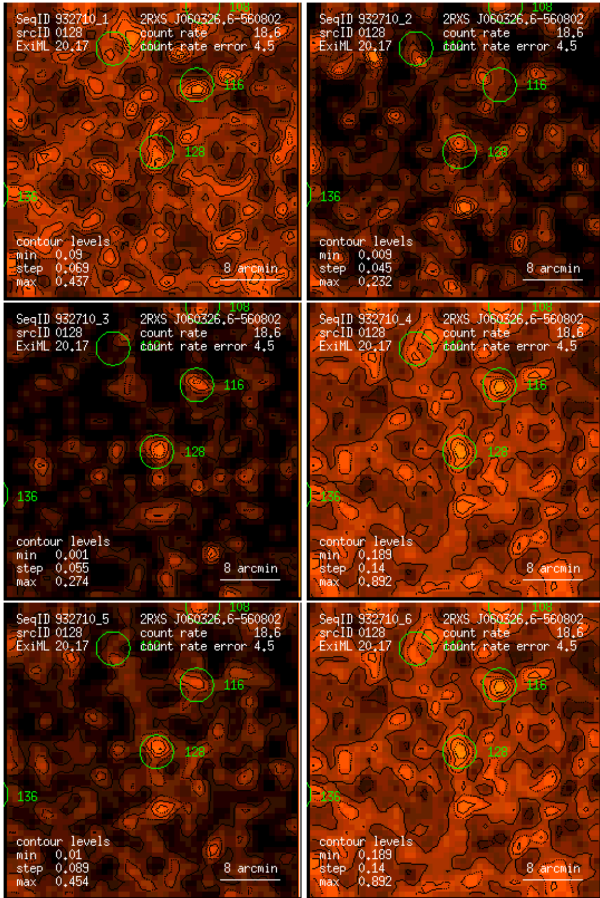
Figure 128: RASS 932710: detection 0128: band rate images, Gaussian filter: (1) PSPC channels 11 – 41, (2) 52 – 90, (3) 91 – 201, (4) 11 – 235, (5) 52 – 201, (6) 11 – 201. Broad band rates in counts/ks. Band rate contour levels in counts/ks/arcmin 2 .
