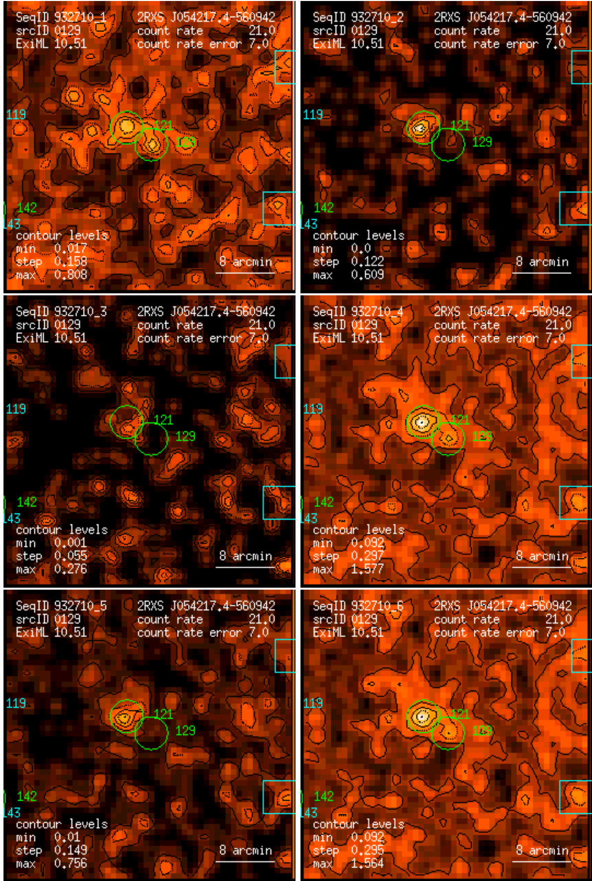
Figure 129: RASS 932710: detection 0129: band rate images, Gaussian filter: (1) PSPC channels 11 – 41, (2) 52 – 90, (3) 91 – 201, (4) 11 – 235, (5) 52 – 201, (6) 11 – 201. Broad band rates in counts/ks. Band rate contour levels in counts/ks/arcmin 2 .
