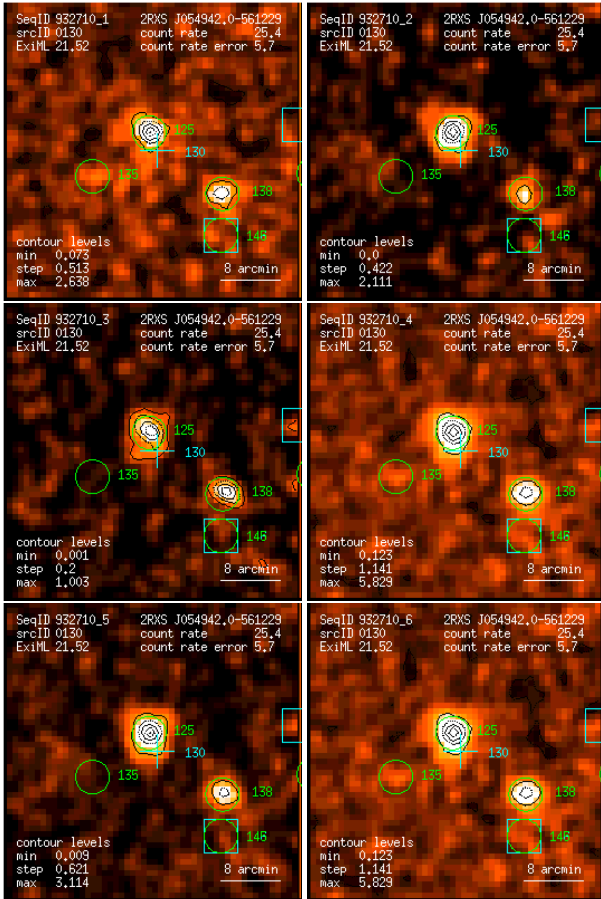
Figure 130: RASS 932710: detection 0130: band rate images, Gaussian filter: (1) PSPC channels 11 – 41, (2) 52 – 90, (3) 91 – 201, (4) 11 – 235, (5) 52 – 201, (6) 11 – 201. Broad band rates in counts/ks. Band rate contour levels in counts/ks/arcmin 2 .
