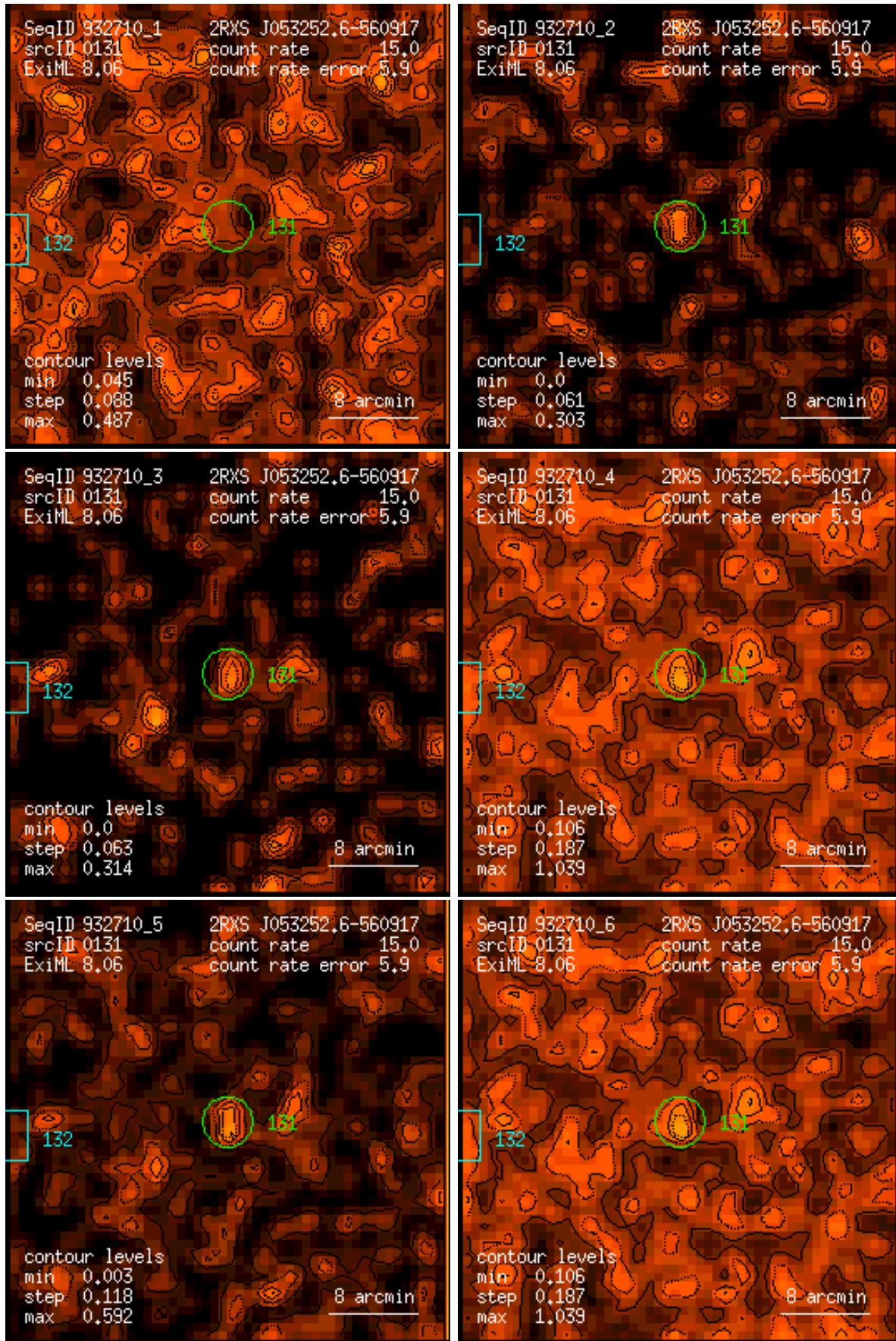
Figure 131: RASS 932710: detection 0131: band rate images, Gaussian filter: (1) PSPC channels 11 – 41, (2) 52 – 90, (3) 91 – 201, (4) 11 – 235, (5) 52 – 201, (6) 11 – 201. Broad band rates in counts/ks. Band rate contour levels in counts/ks/arcmin 2 .
