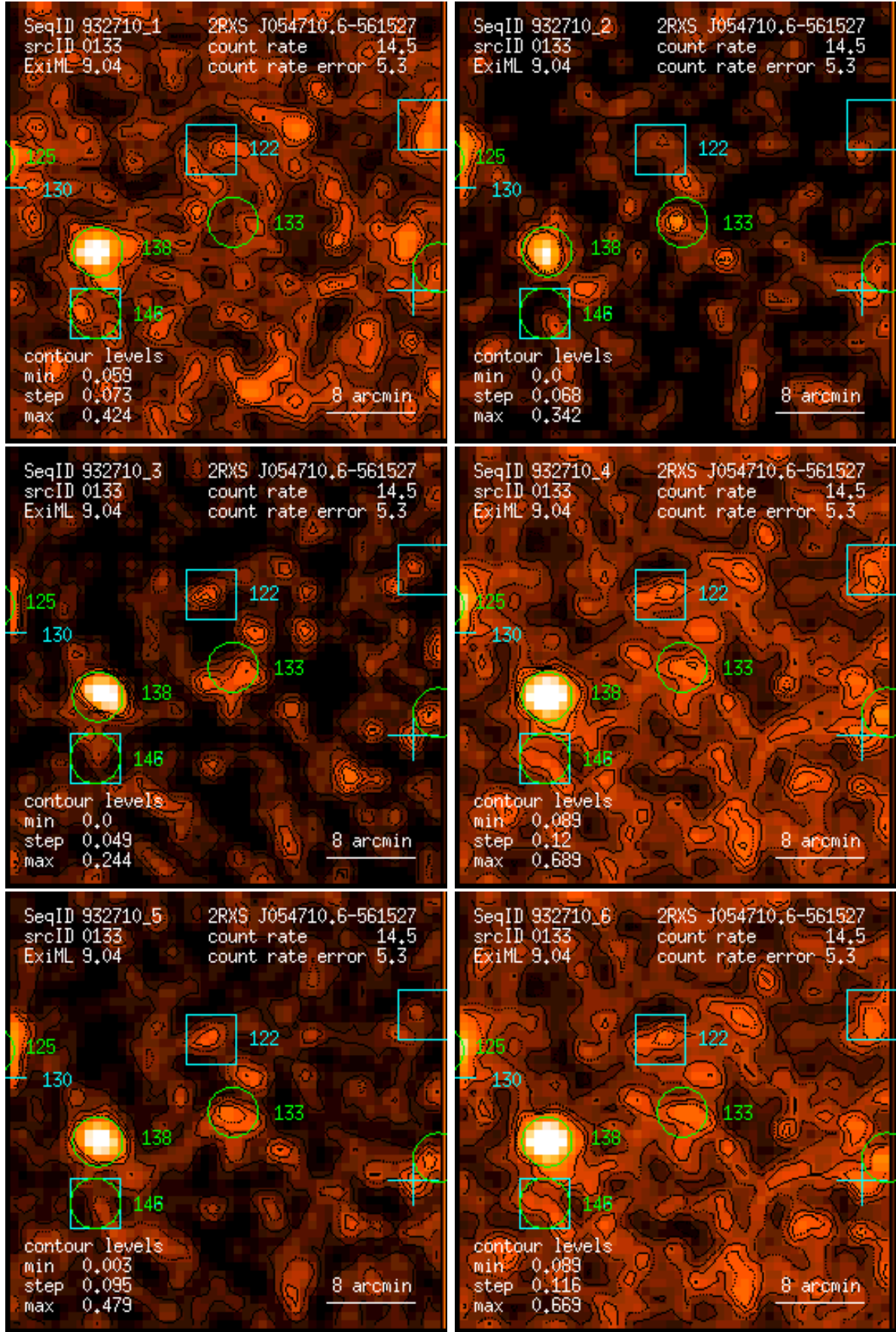
Figure 133: RASS 932710: detection 0133: band rate images, Gaussian filter: (1) PSPC channels 11 – 41, (2) 52 – 90, (3) 91 – 201, (4) 11 – 235, (5) 52 – 201, (6) 11 – 201. Broad band rates in counts/ks. Band rate contour levels in counts/ks/arcmin 2 .
