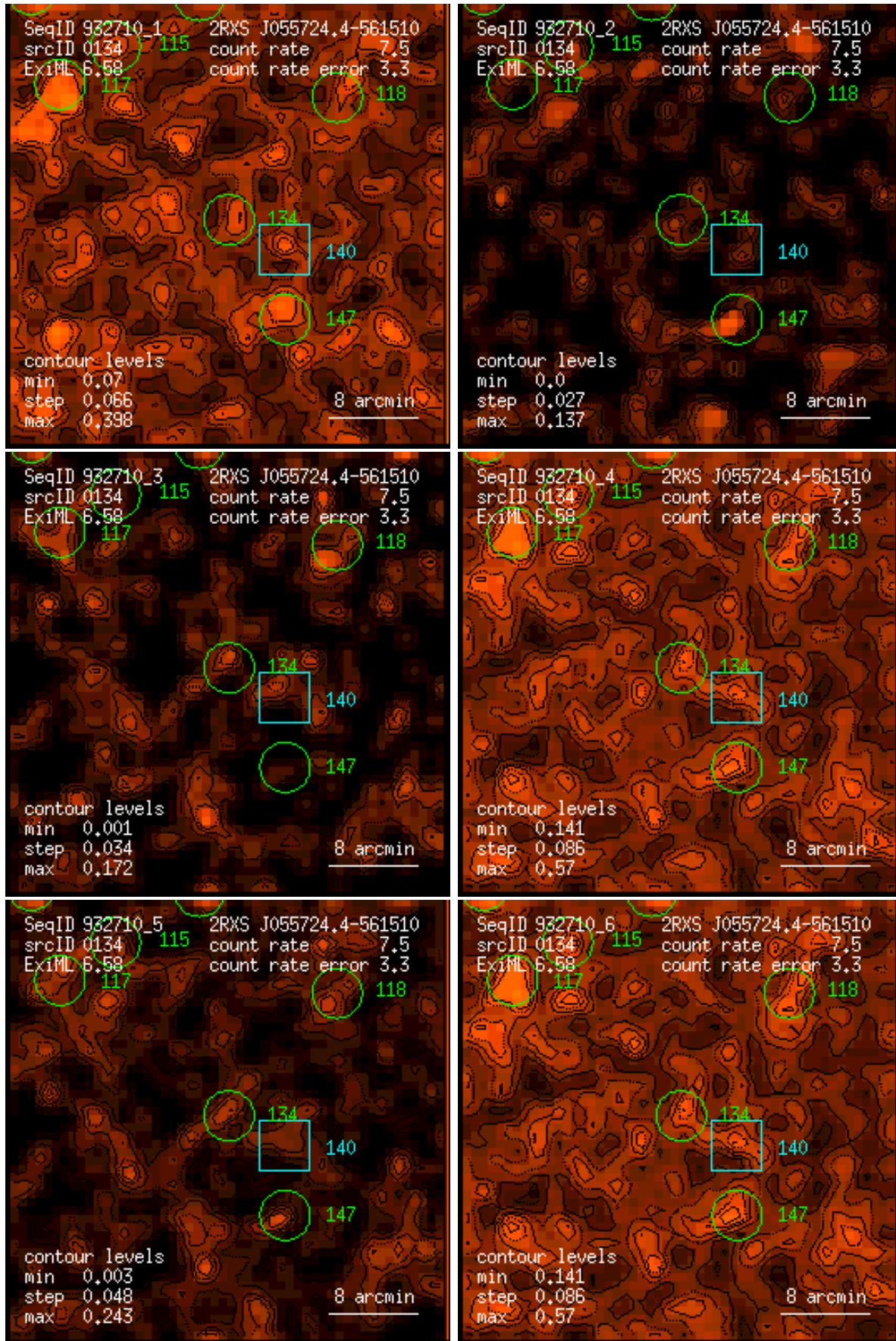
Figure 134: RASS 932710: detection 0134: band rate images, Gaussian filter: (1) PSPC channels 11 – 41, (2) 52 – 90, (3) 91 – 201, (4) 11 – 235, (5) 52 – 201, (6) 11 – 201. Broad band rates in counts/ks. Band rate contour levels in counts/ks/arcmin 2 .
