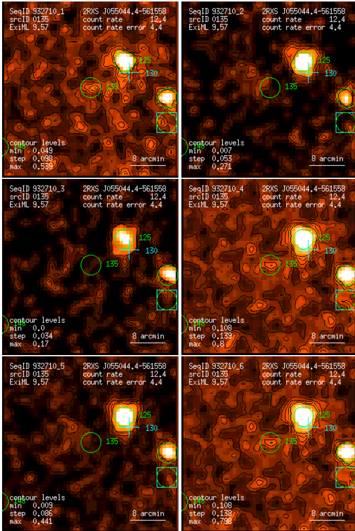
Figure 135: RASS 932710: detection 0135: band rate images, Gaussian filter: (1) PSPC channels 11 – 41, (2) 52 – 90, (3) 91 – 201, (4) 11 – 235, (5) 52 – 201, (6) 11 – 201. Broad band rates in counts/ks. Band rate contour levels in counts/ks/arcmin 2 .
