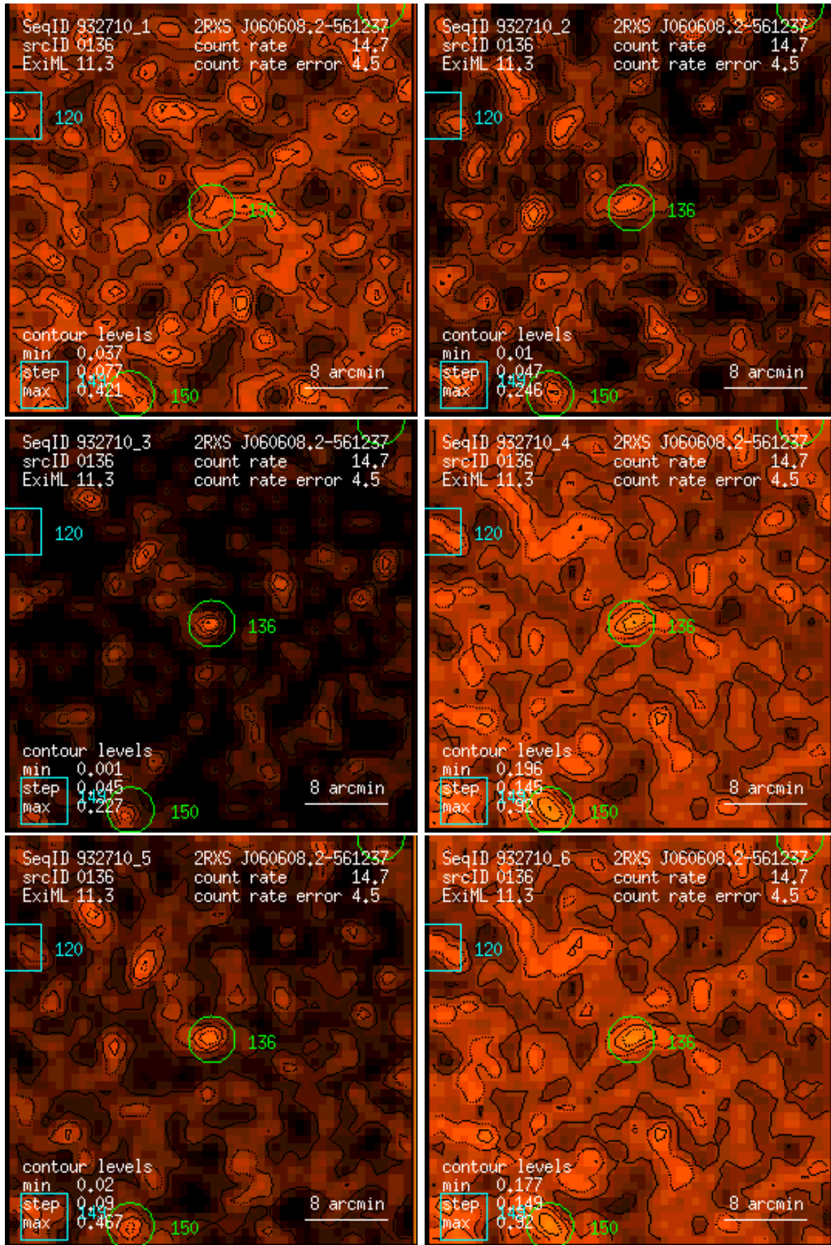
Figure 136: RASS 932710: detection 0136: band rate images, Gaussian filter: (1) PSPC channels 11 – 41, (2) 52 – 90, (3) 91 – 201, (4) 11 – 235, (5) 52 – 201, (6) 11 – 201. Broad band rates in counts/ks. Band rate contour levels in counts/ks/arcmin 2 .
