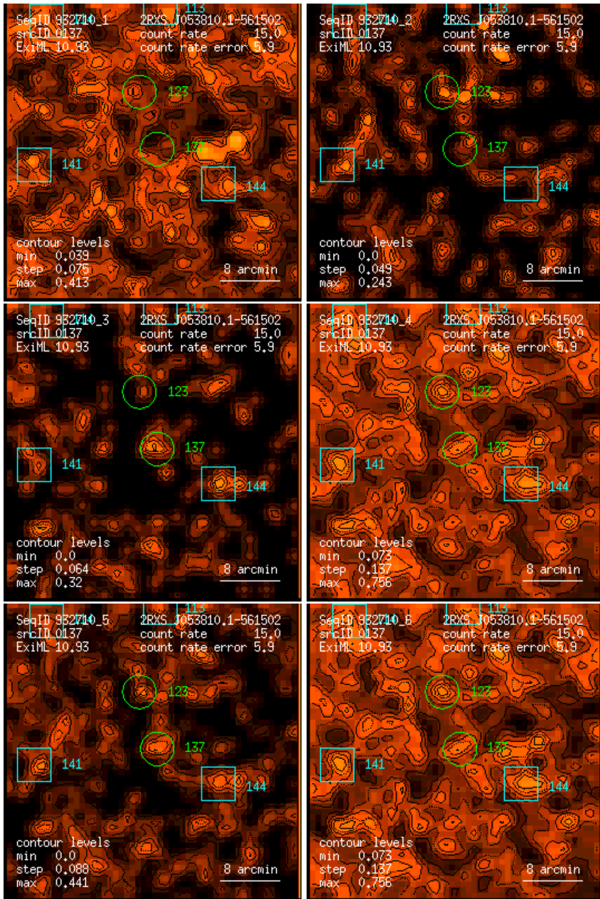
Figure 137: RASS 932710: detection 0137: band rate images, Gaussian filter: (1) PSPC channels 11 – 41, (2) 52 – 90, (3) 91 – 201, (4) 11 – 235, (5) 52 – 201, (6) 11 – 201. Broad band rates in counts/ks. Band rate contour levels in counts/ks/arcmin 2 .
