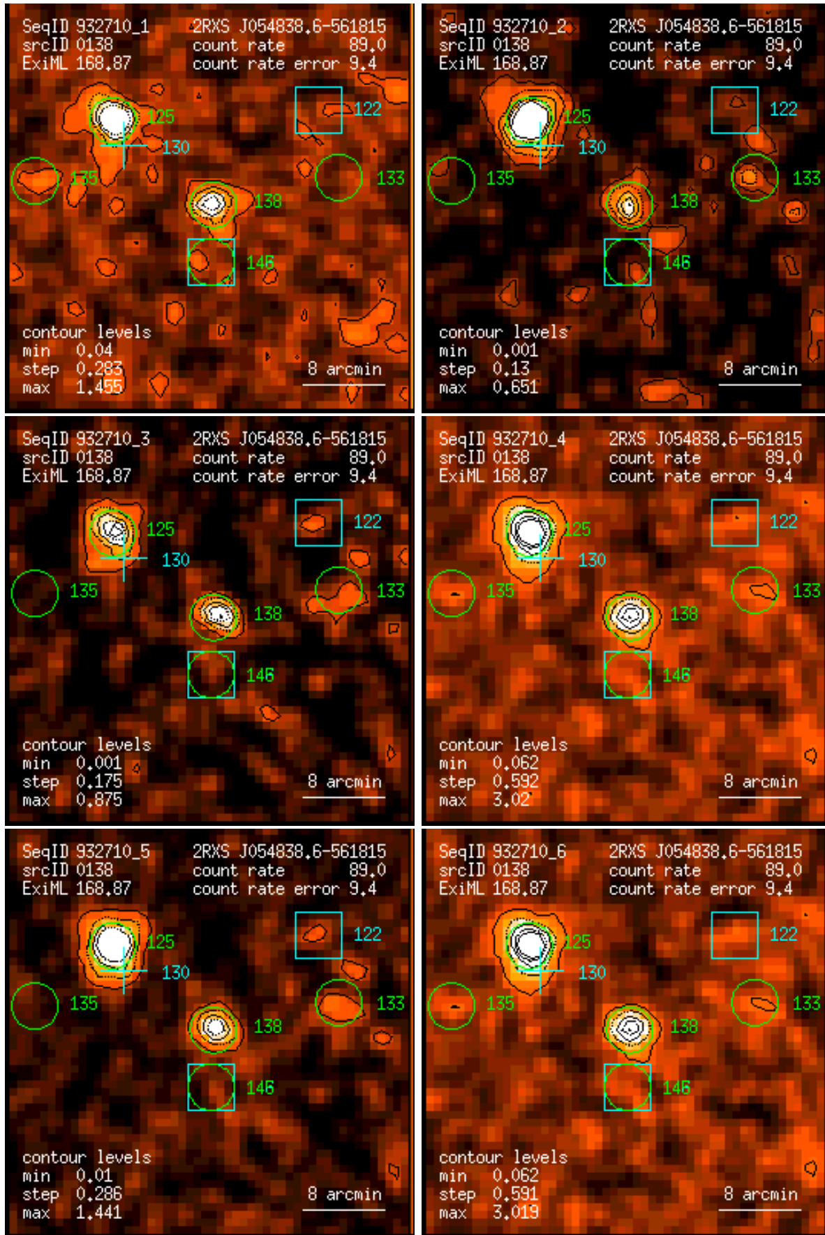
Figure 138: RASS 932710: detection 0138: band rate images, Gaussian filter: (1) PSPC channels 11 – 41, (2) 52 – 90, (3) 91 – 201, (4) 11 – 235, (5) 52 – 201, (6) 11 – 201. Broad band rates in counts/ks. Band rate contour levels in counts/ks/arcmin 2 .
