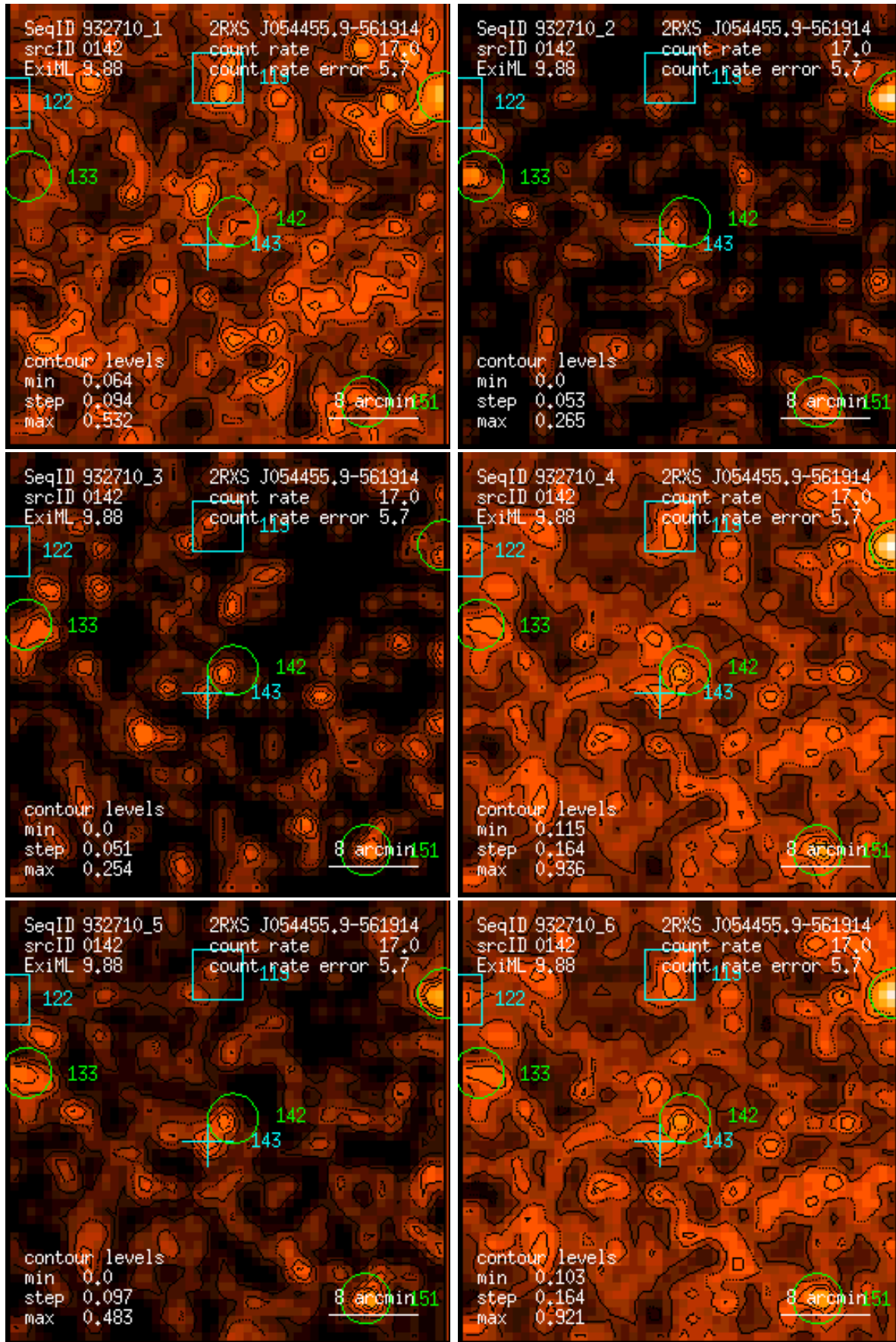
Figure 142: RASS 932710: detection 0142: band rate images, Gaussian filter: (1) PSPC channels 11 – 41, (2) 52 – 90, (3) 91 – 201, (4) 11 – 235, (5) 52 – 201, (6) 11 – 201. Broad band rates in counts/ks. Band rate contour levels in counts/ks/arcmin 2 .
