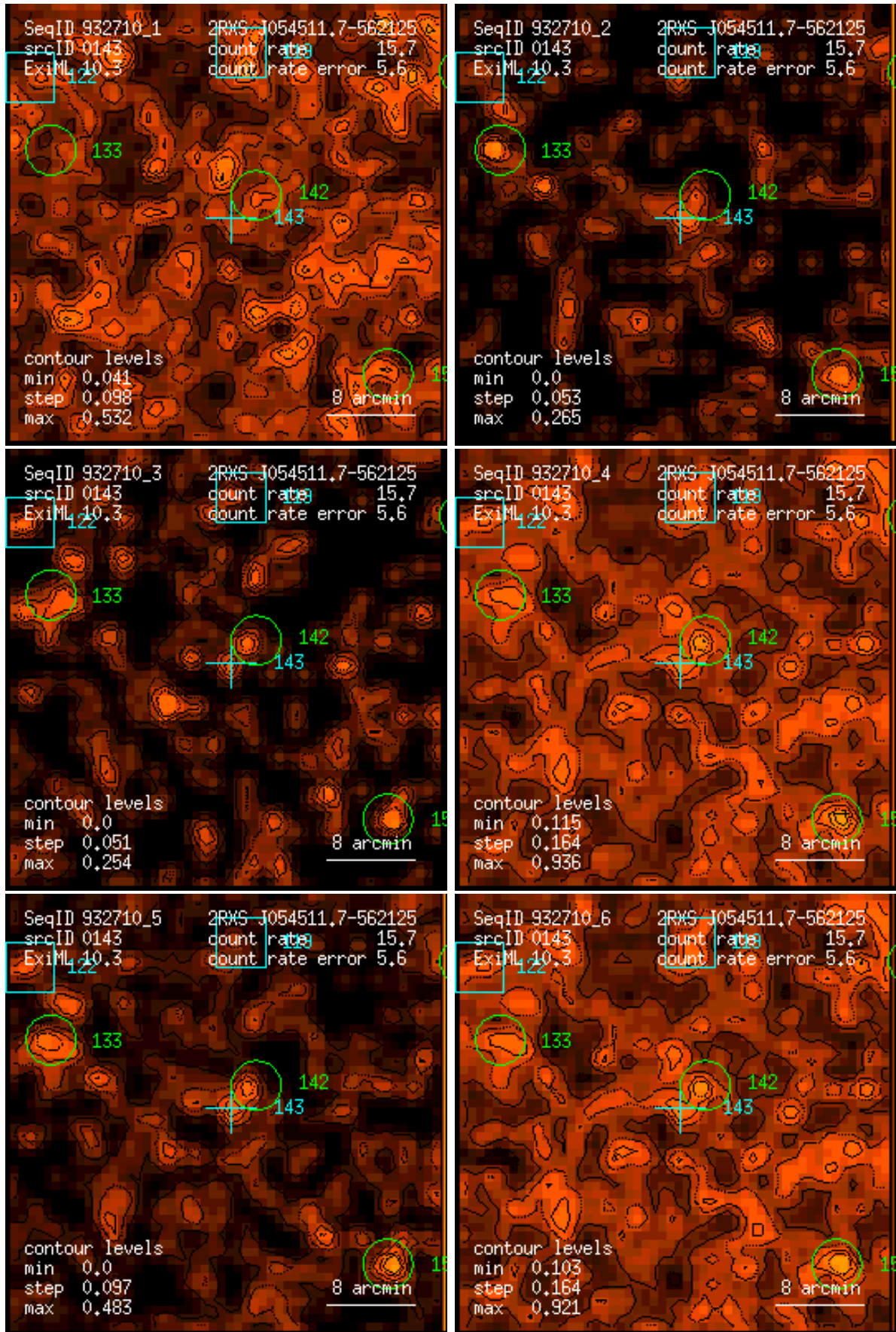
Figure 143: RASS 932710: detection 0143: band rate images, Gaussian filter: (1) PSPC channels 11 – 41, (2) 52 – 90, (3) 91 – 201, (4) 11 – 235, (5) 52 – 201, (6) 11 – 201. Broad band rates in counts/ks. Band rate contour levels in counts/ks/arcmin 2 .
