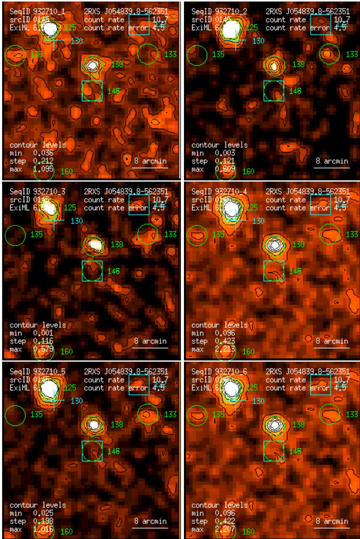
Figure 145: RASS 932710: detection 0145: band rate images, Gaussian filter: (1) PSPC channels 11 – 41, (2) 52 – 90, (3) 91 – 201, (4) 11 – 235, (5) 52 – 201, (6) 11 – 201. Broad band rates in counts/ks. Band rate contour levels in counts/ks/arcmin 2 .
