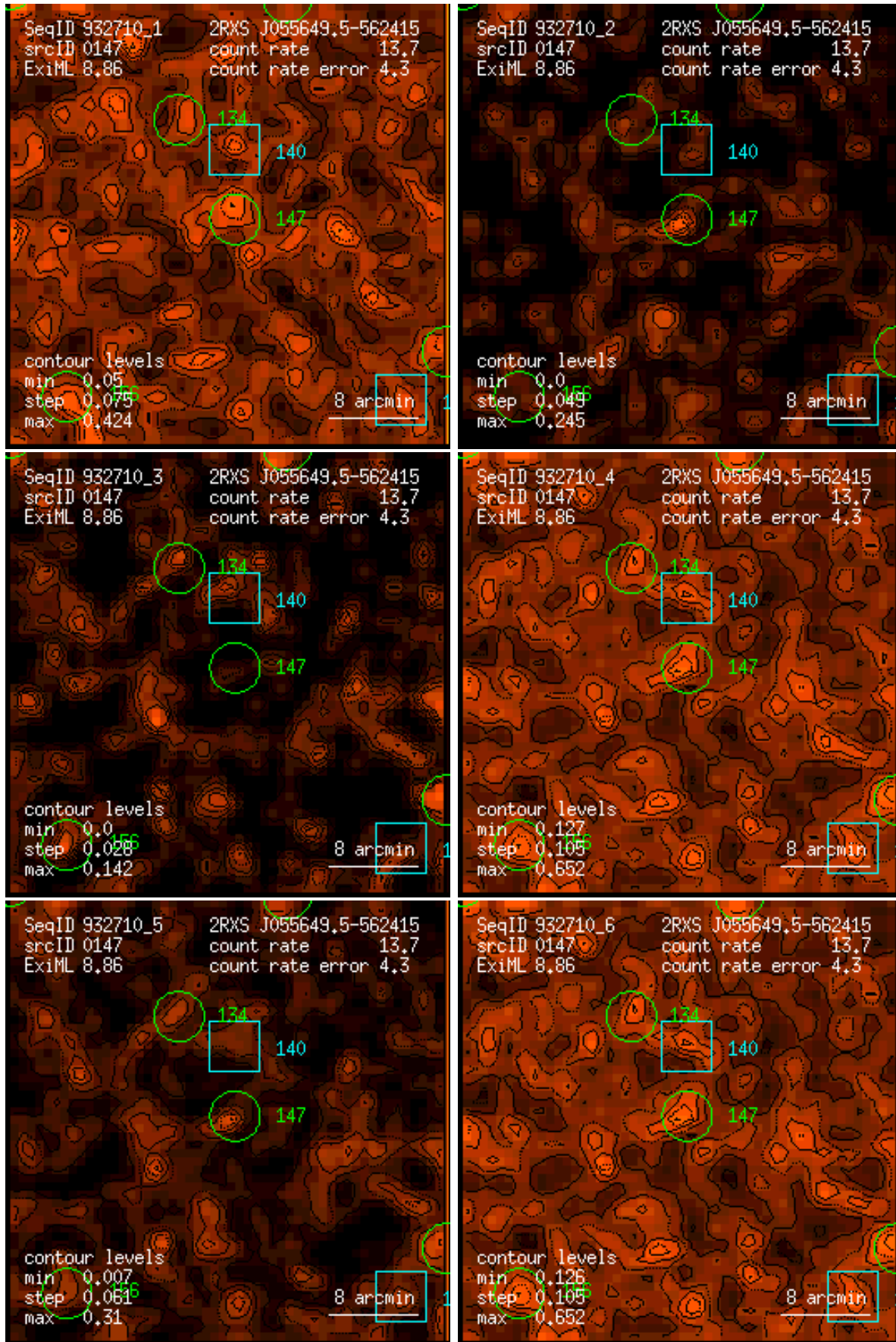
Figure 147: RASS 932710: detection 0147: band rate images, Gaussian filter: (1) PSPC channels 11 – 41, (2) 52 – 90, (3) 91 – 201, (4) 11 – 235, (5) 52 – 201, (6) 11 – 201. Broad band rates in counts/ks. Band rate contour levels in counts/ks/arcmin 2 .
