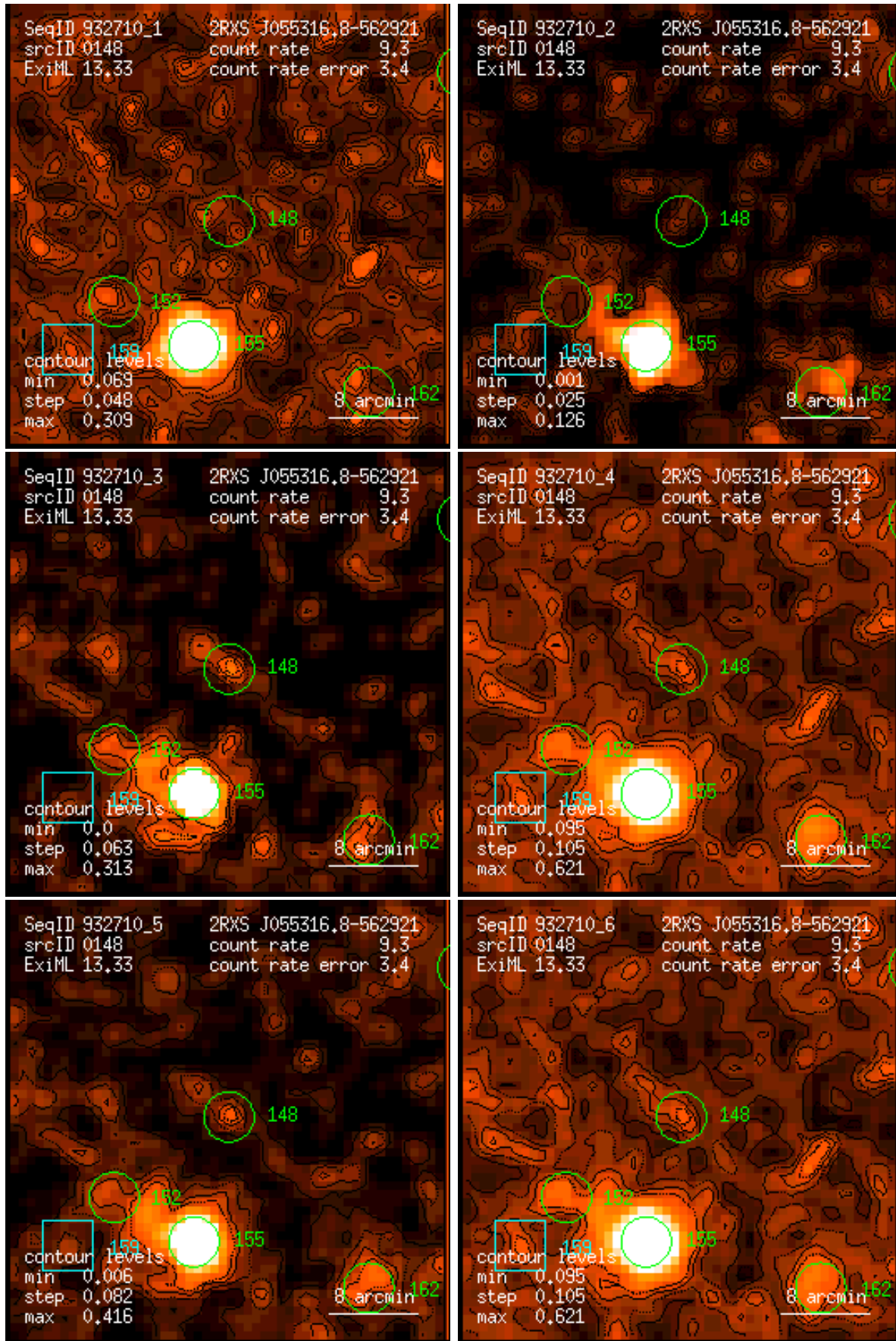
Figure 148: RASS 932710: detection 0148: band rate images, Gaussian filter: (1) PSPC channels 11 – 41, (2) 52 – 90, (3) 91 – 201, (4) 11 – 235, (5) 52 – 201, (6) 11 – 201. Broad band rates in counts/ks. Band rate contour levels in counts/ks/arcmin 2 .
