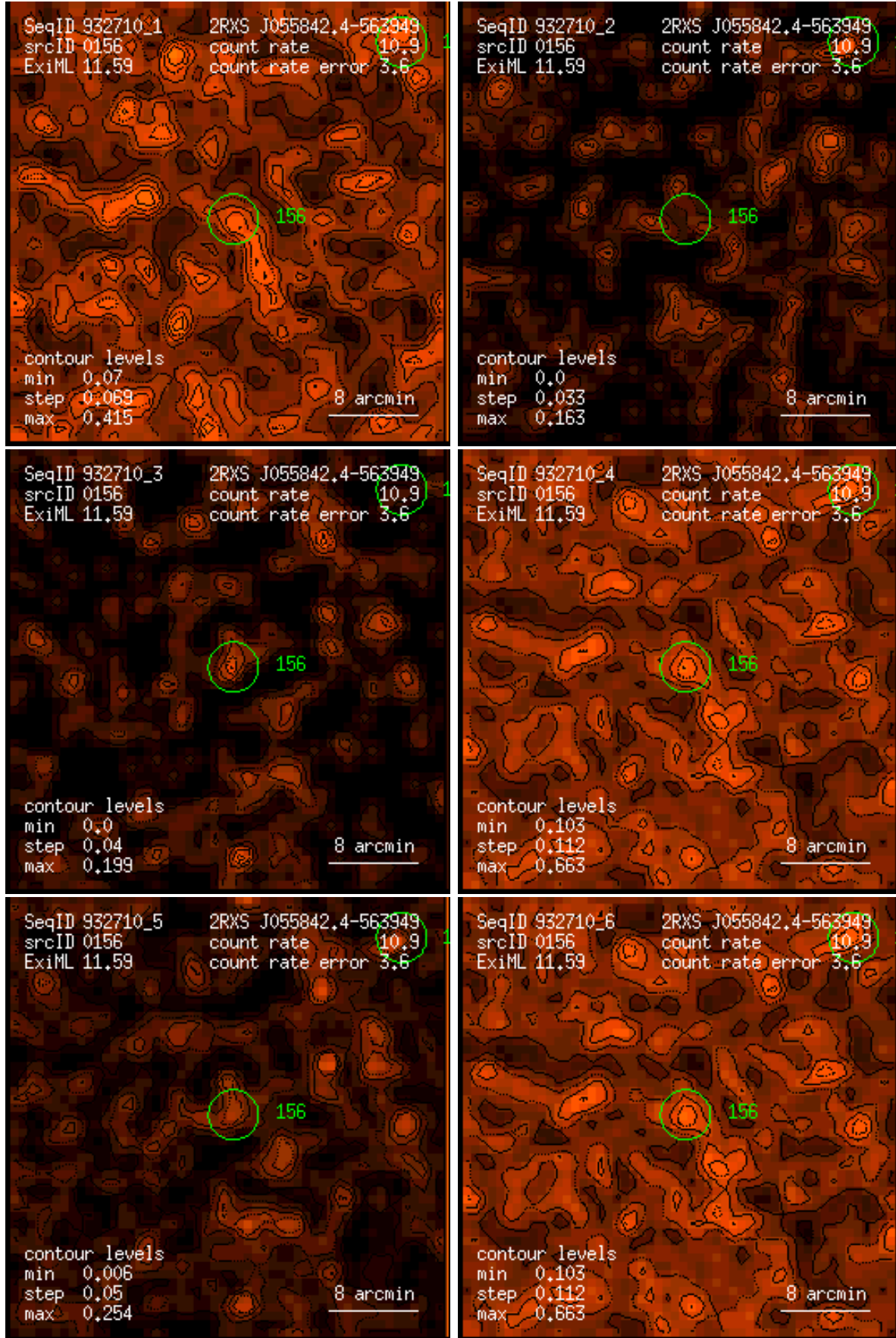
Figure 156: RASS 932710: detection 0156: band rate images, Gaussian filter: (1) PSPC channels 11 – 41, (2) 52 – 90, (3) 91 – 201, (4) 11 – 235, (5) 52 – 201, (6) 11 – 201. Broad band rates in counts/ks. Band rate contour levels in counts/ks/arcmin 2 .
