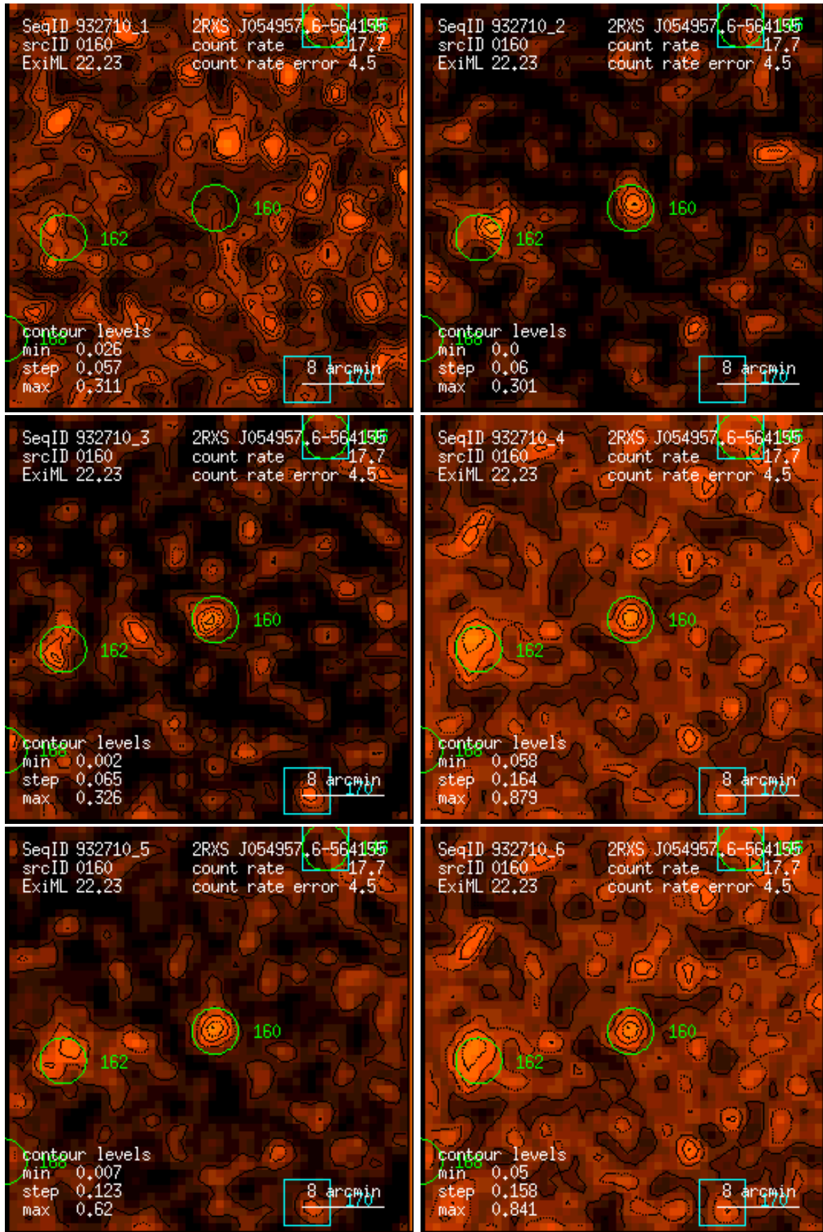
Figure 160: RASS 932710: detection 0160: band rate images, Gaussian filter: (1) PSPC channels 11 – 41, (2) 52 – 90, (3) 91 – 201, (4) 11 – 235, (5) 52 – 201, (6) 11 – 201. Broad band rates in counts/ks. Band rate contour levels in counts/ks/arcmin 2 .
