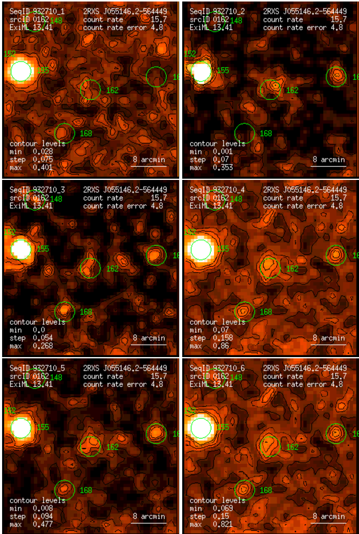
Figure 162: RASS 932710: detection 0162: band rate images, Gaussian filter: (1) PSPC channels 11 – 41, (2) 52 – 90, (3) 91 – 201, (4) 11 – 235, (5) 52 – 201, (6) 11 – 201. Broad band rates in counts/ks. Band rate contour levels in counts/ks/arcmin 2 .
