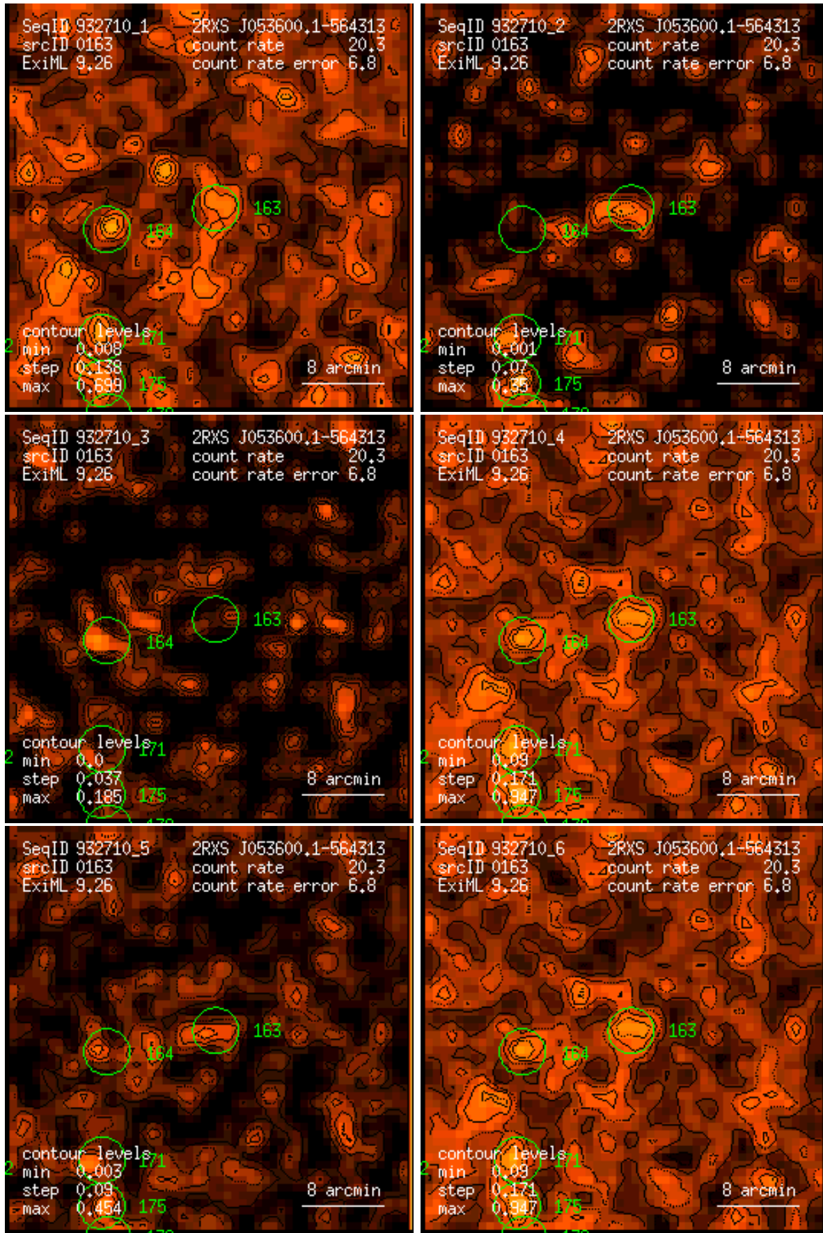
Figure 163: RASS 932710: detection 0163: band rate images, Gaussian filter: (1) PSPC channels 11 – 41, (2) 52 – 90, (3) 91 – 201, (4) 11 – 235, (5) 52 – 201, (6) 11 – 201. Broad band rates in counts/ks. Band rate contour levels in counts/ks/arcmin 2 .
