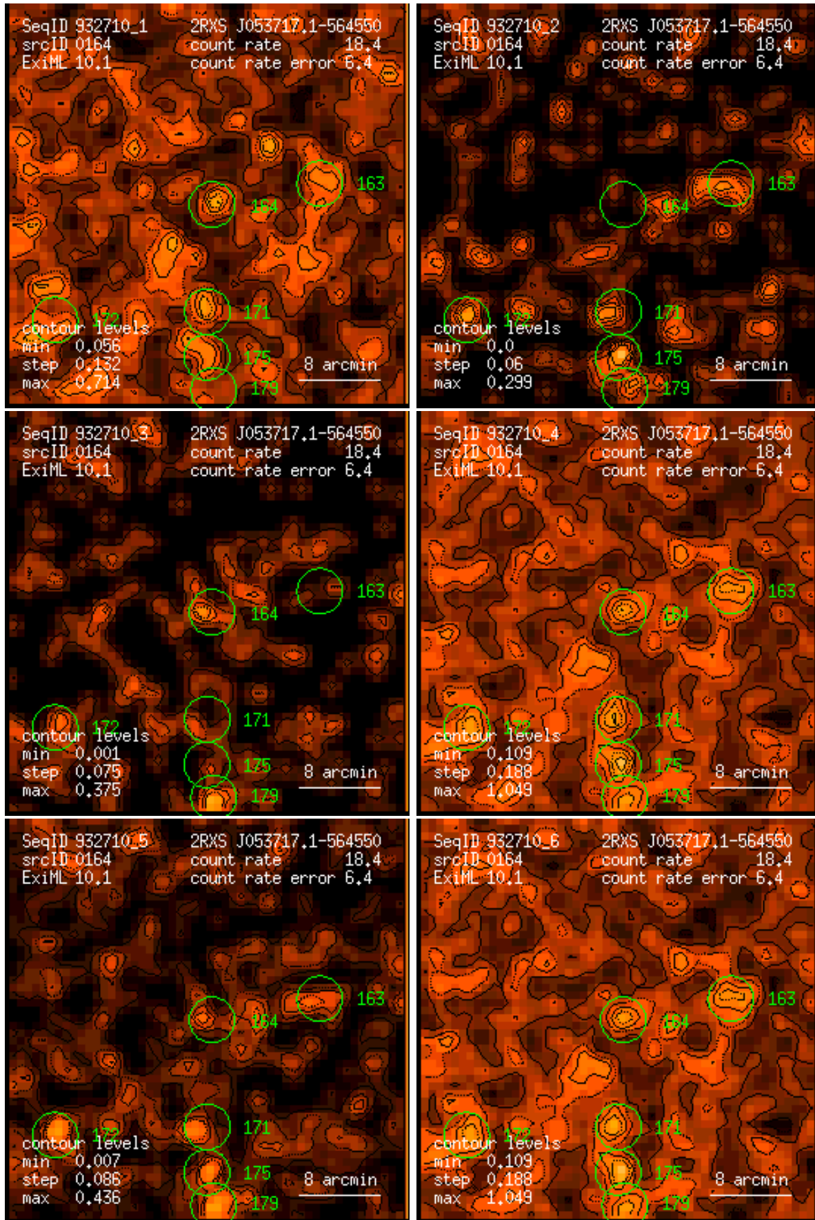
Figure 164: RASS 932710: detection 0164: band rate images, Gaussian filter: (1) PSPC channels 11 – 41, (2) 52 – 90, (3) 91 – 201, (4) 11 – 235, (5) 52 – 201, (6) 11 – 201. Broad band rates in counts/ks. Band rate contour levels in counts/ks/arcmin 2 .
