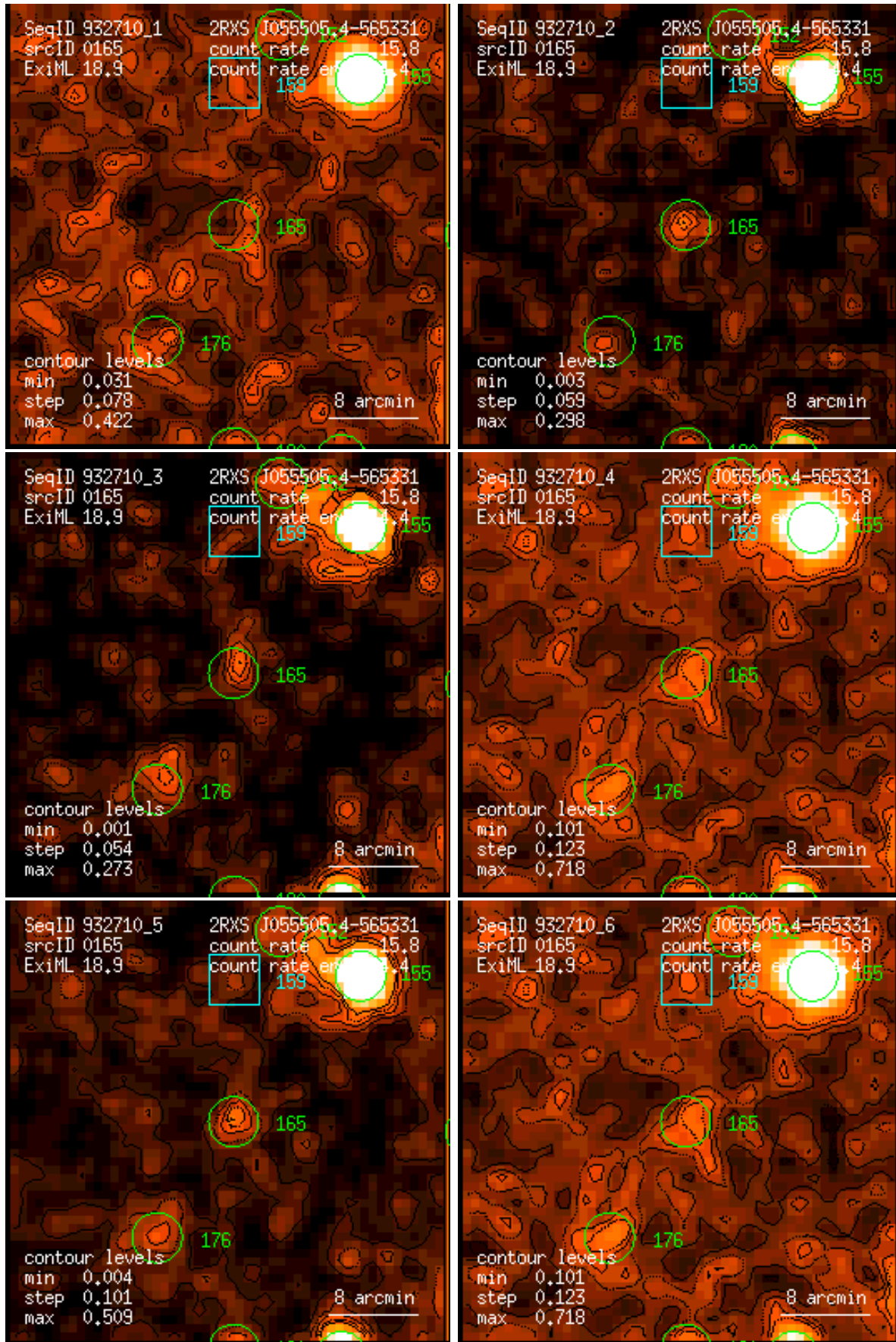
Figure 165: RASS 932710: detection 0165: band rate images, Gaussian filter: (1) PSPC channels 11 – 41, (2) 52 – 90, (3) 91 – 201, (4) 11 – 235, (5) 52 – 201, (6) 11 – 201. Broad band rates in counts/ks. Band rate contour levels in counts/ks/arcmin 2 .
